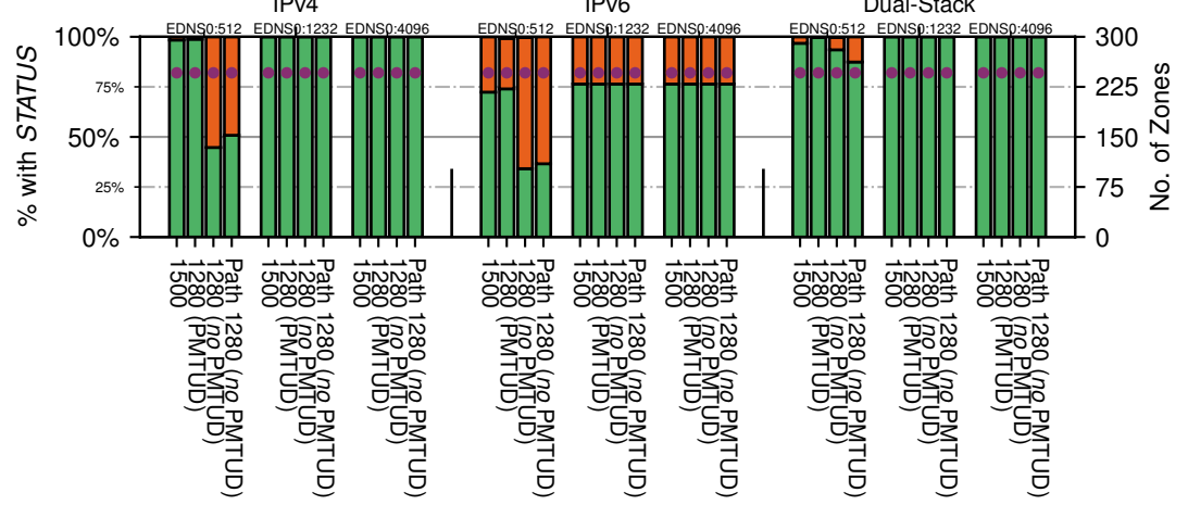
All Zones with DNSSEC for '.it'
