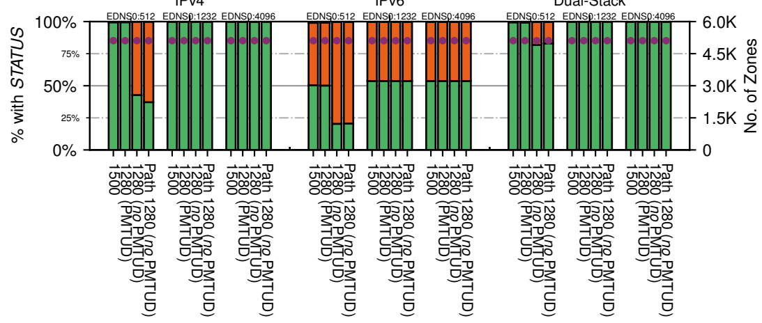
All Zones without DNSSEC for '.it'
