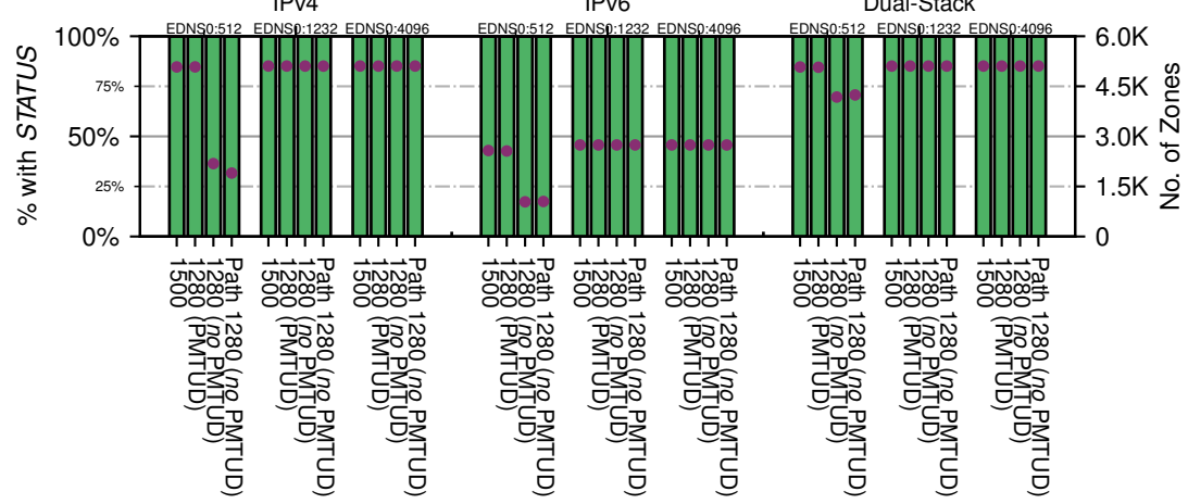
All Zones without DNSSEC returning NOERROR for '.it'
