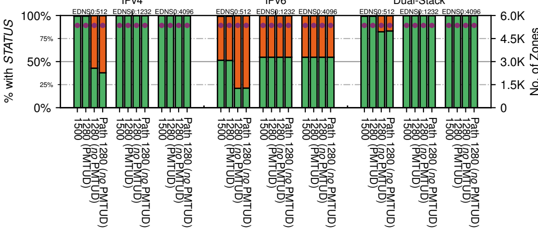
All Zones with EDNS0 for '.it'
