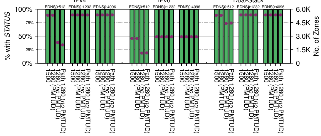
All Zones returning NOERROR for '.it'
