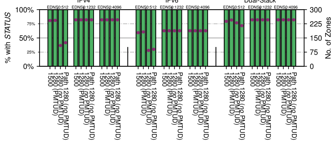
All Zones with DNSSEC returning NOERROR for '.it'
