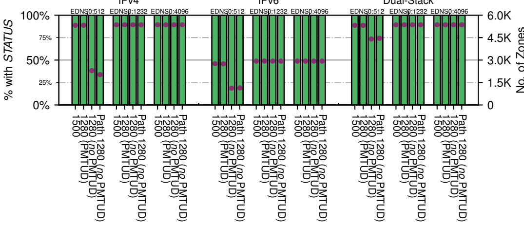
All Zones with EDNS0 returning NOERROR for '.it'
