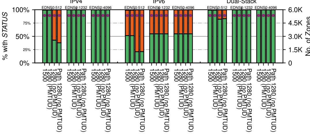
All Zones for '.it'
