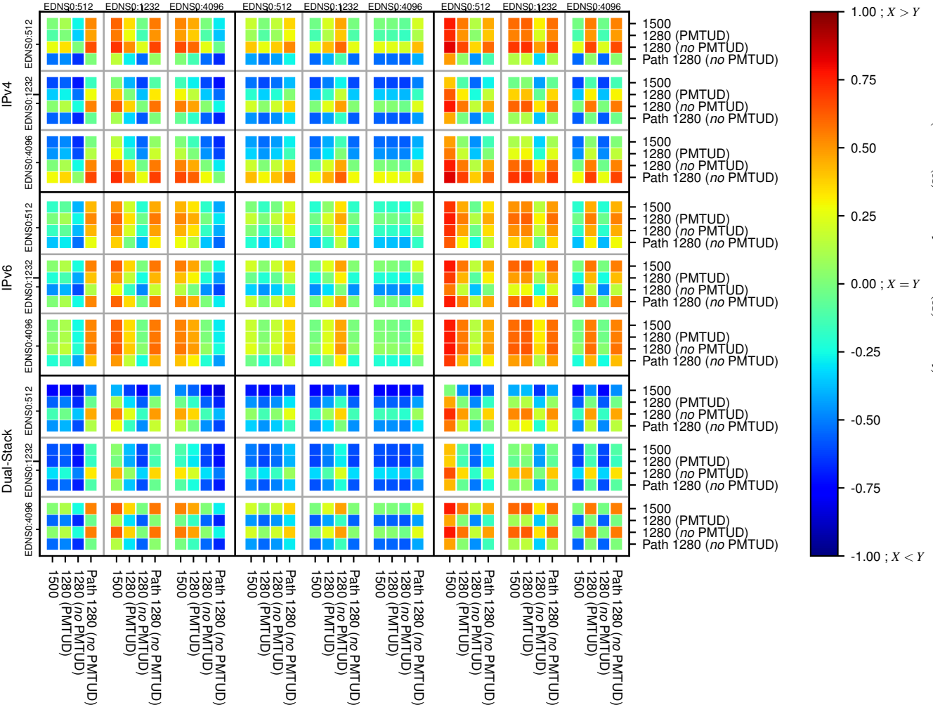
All Zones returning NOERROR for '.fr'
