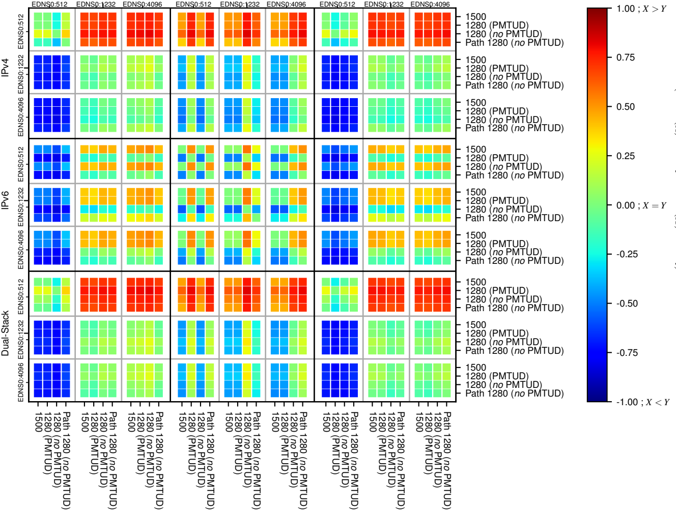
All Zones with DNSSEC returning NOERROR for '.fr'
