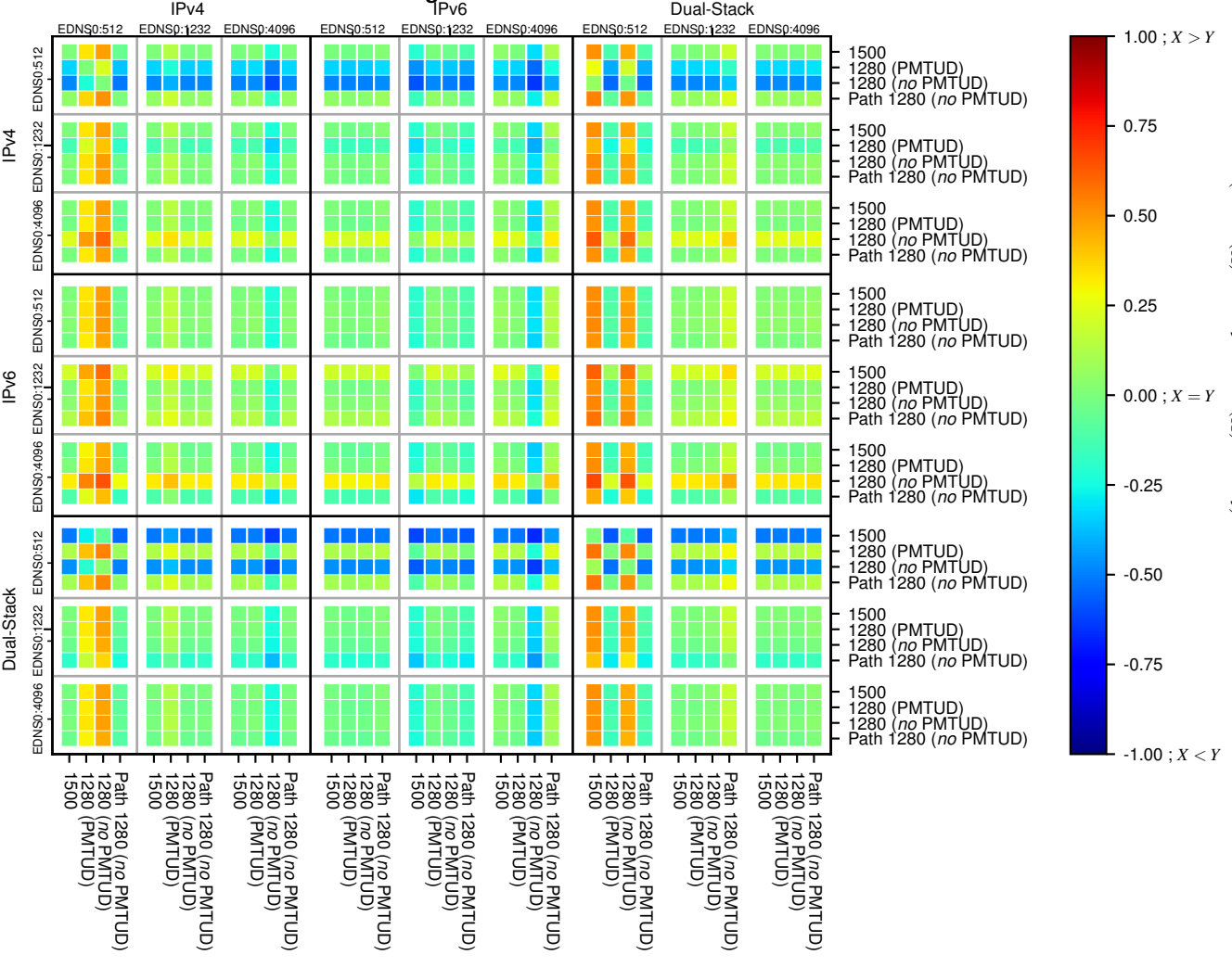
All Zones without DNSSEC returning NOERROR for '.fr'
