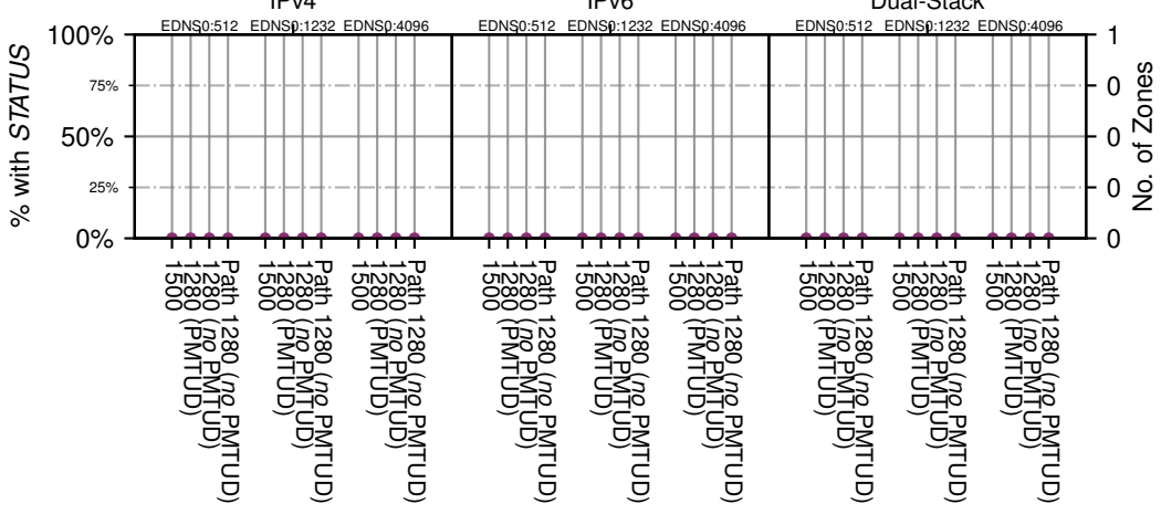
All Zones without EDNS0 for '.br'
