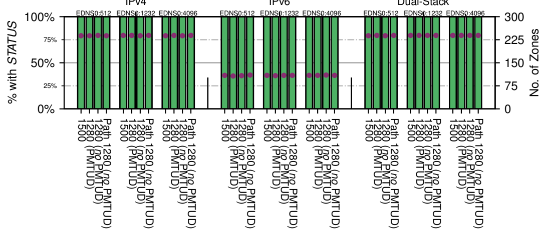
All Zones without DNSSEC returning NOERROR for '.br'
