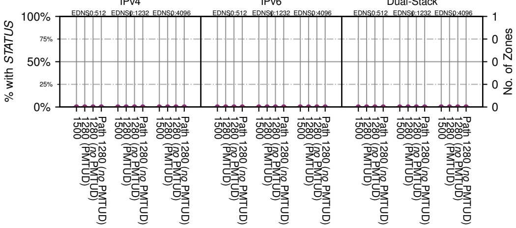
All Zones without EDNS0 returning NOERROR for '.br'
