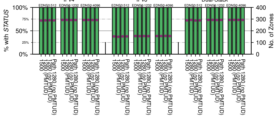
All Zones returning NOERROR for '.br'
