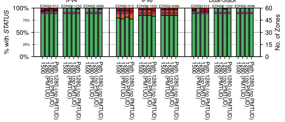
All Zones with DNSSEC for '.br'
