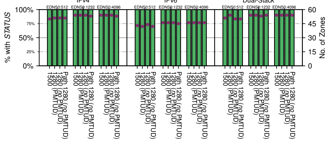
All Zones with DNSSEC returning NOERROR for '.br'
