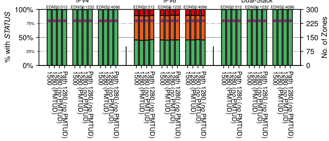
All Zones without DNSSEC for '.br'
