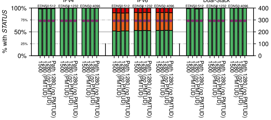
All Zones with EDNS0 for '.br'
