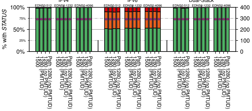
All Zones for '.br'
