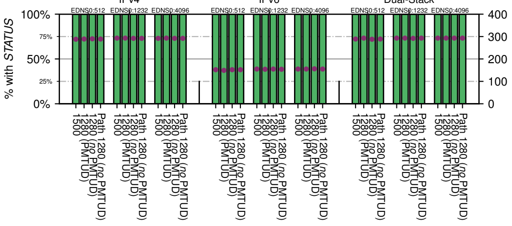
All Zones with EDNS0 returning NOERROR for '.br'
