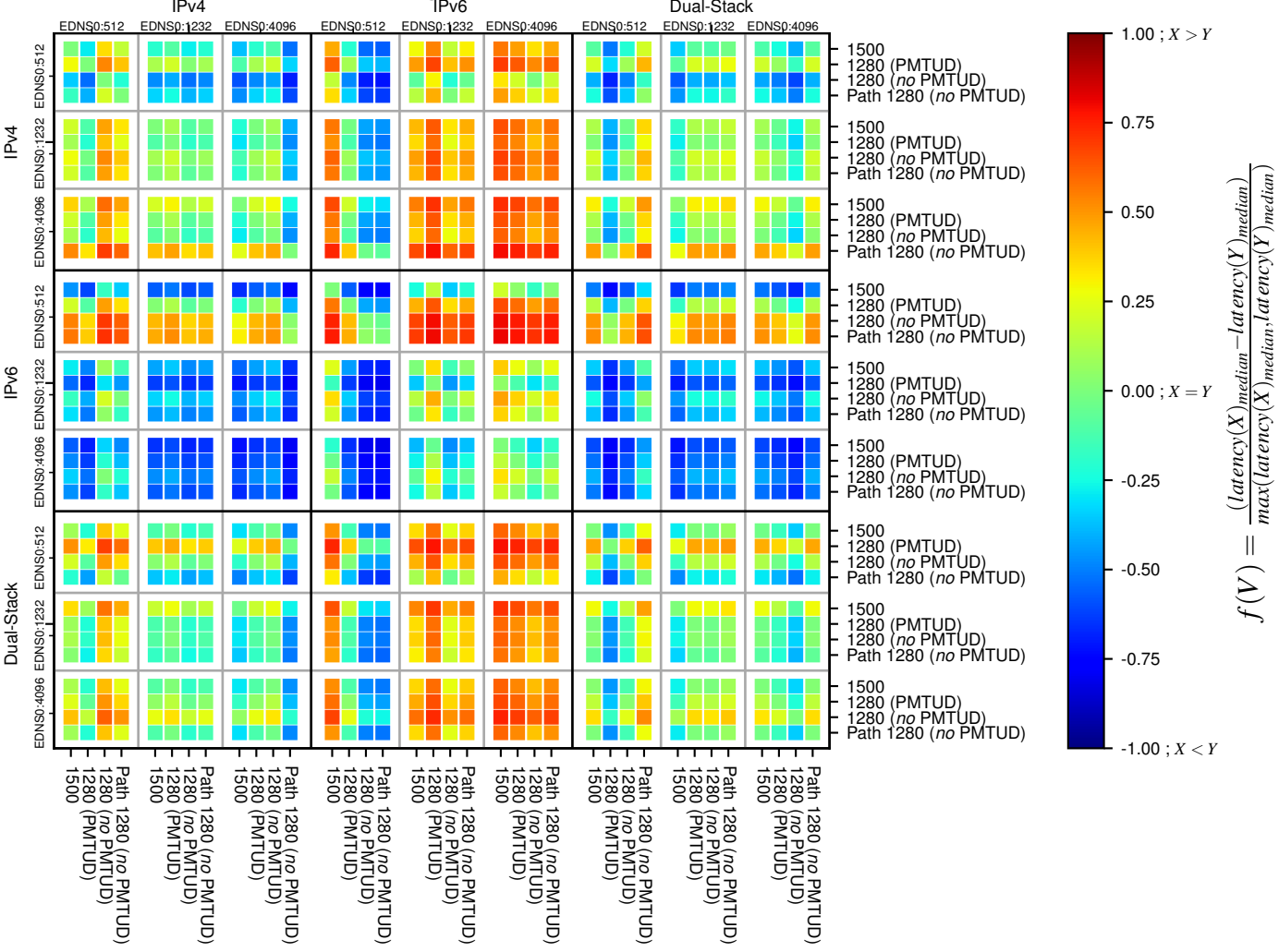
All Zones without DNSSEC returning NOERROR for '.se'
