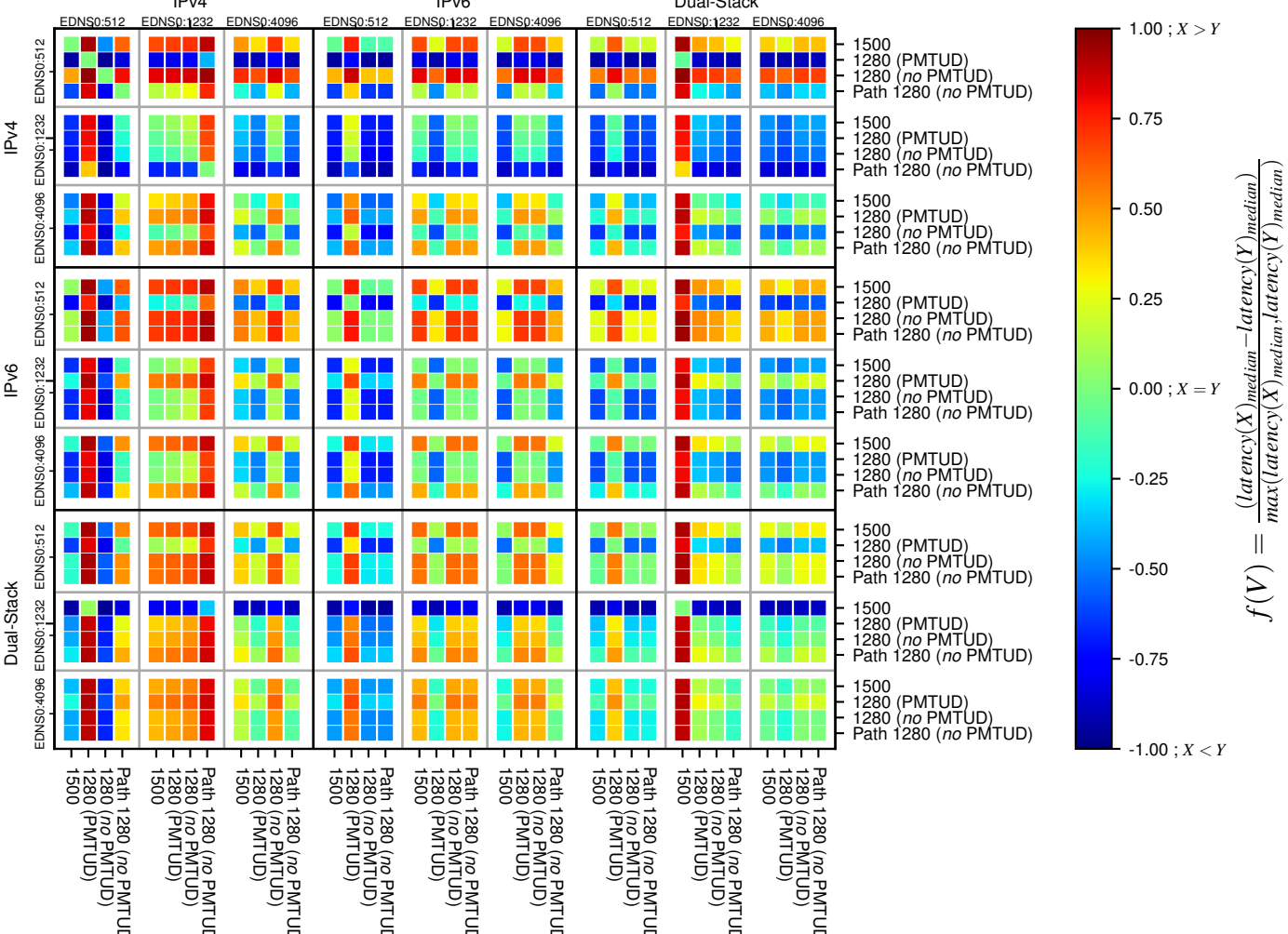
All Zones returning NOERROR for '.se'
