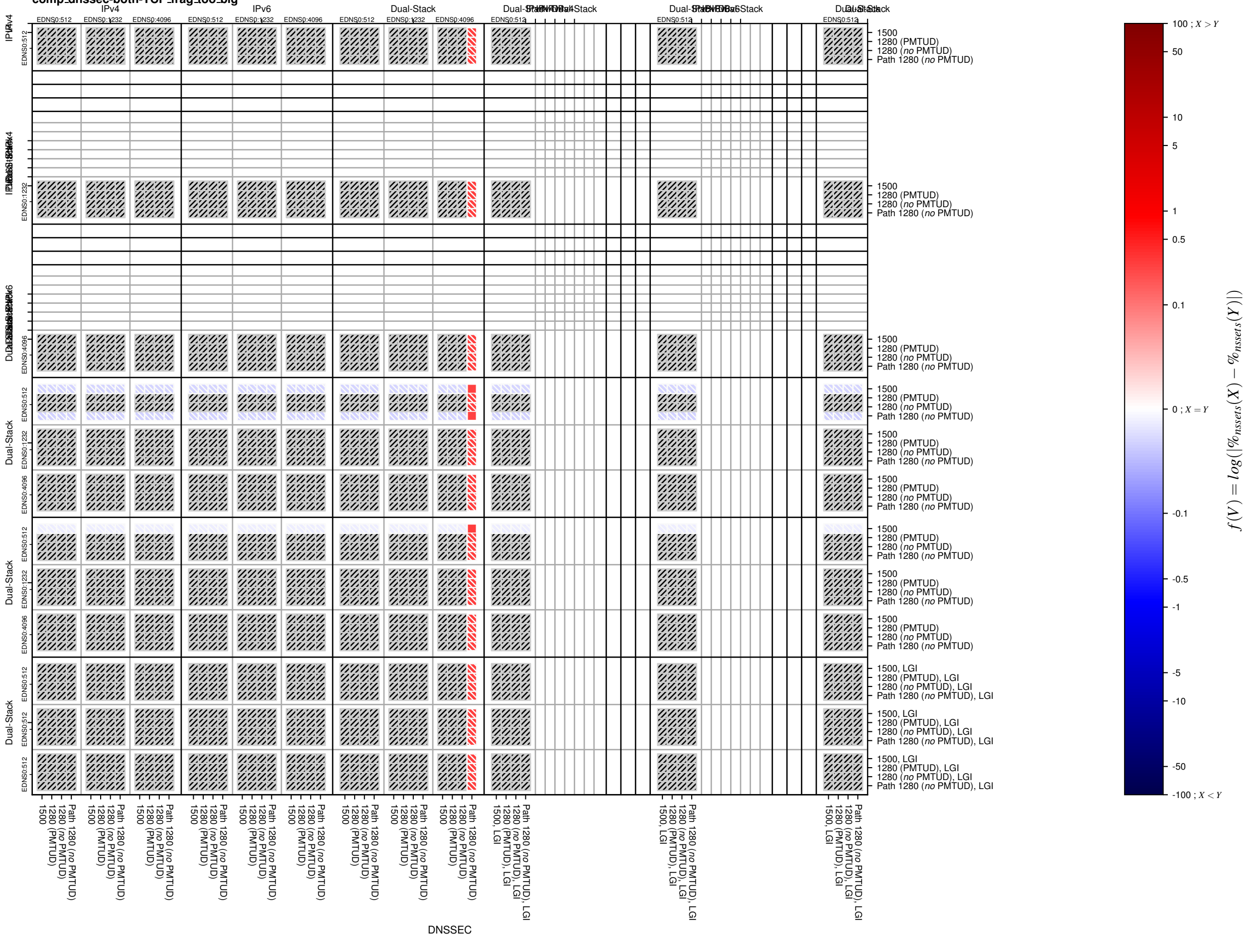
comp_dnssec-both-TCP_frag_too_big
