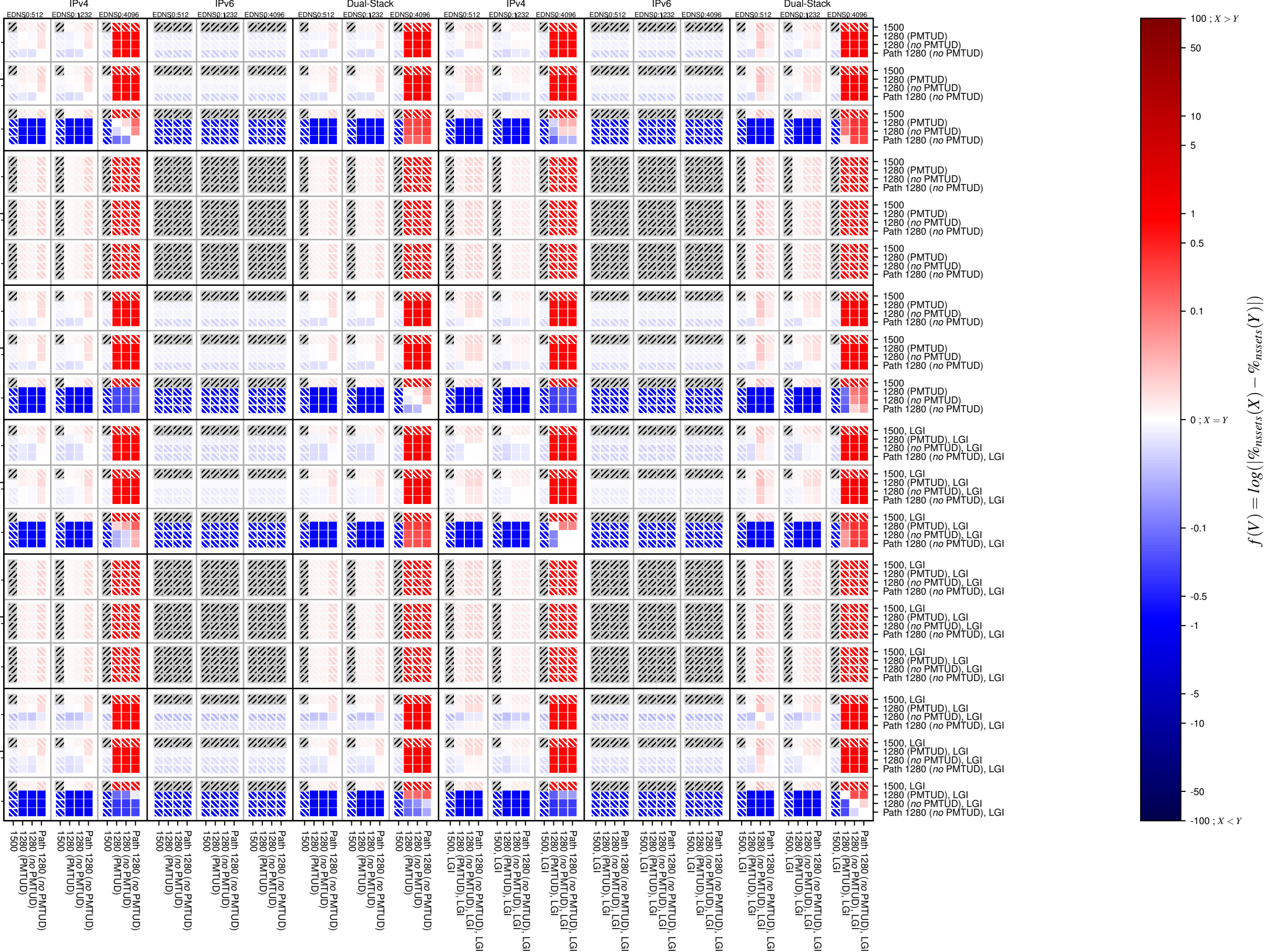
dnssec-v4-UDP_packet_too_big
