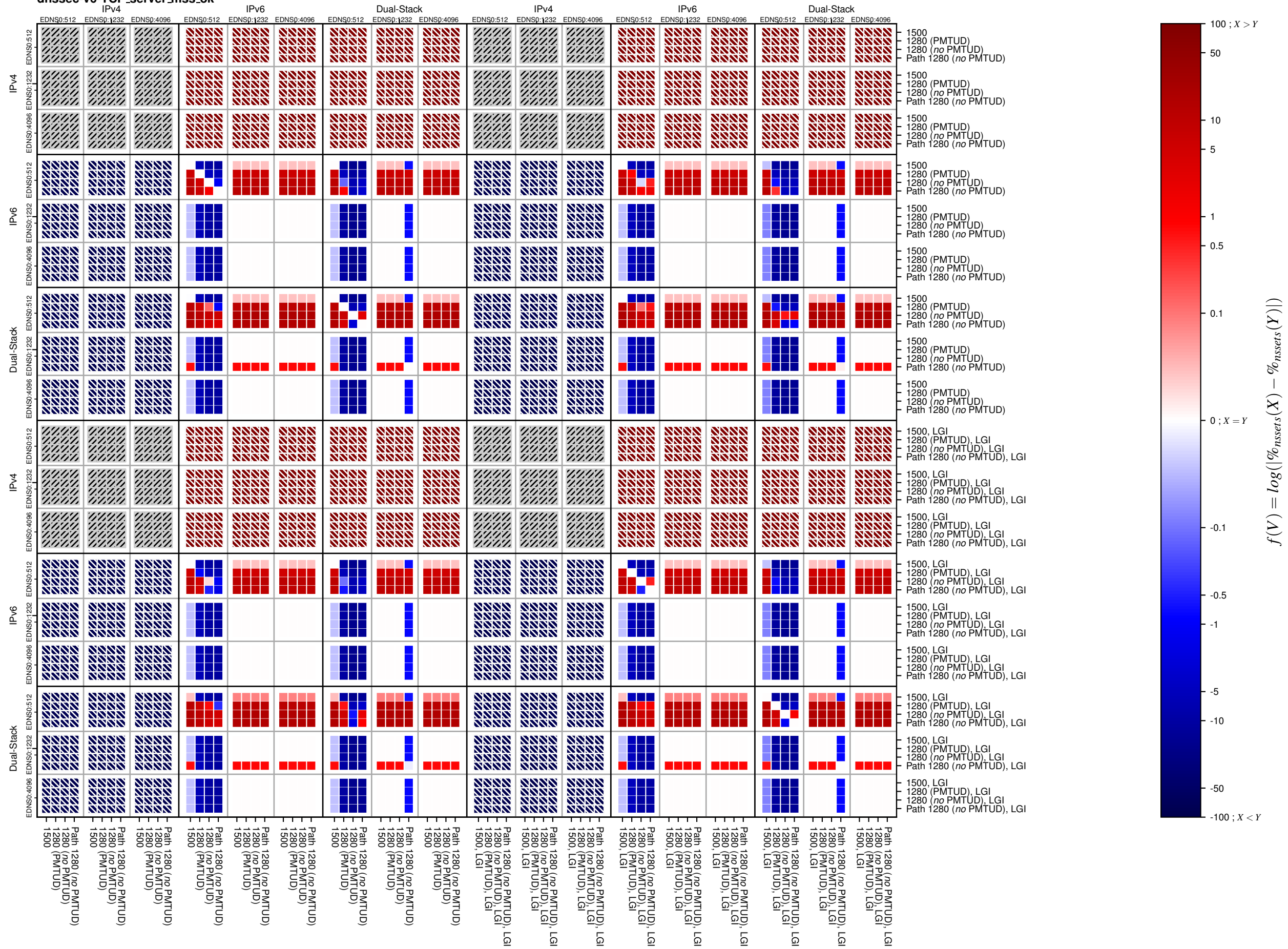
dnssec-v6-TCP_server_mss_ok
