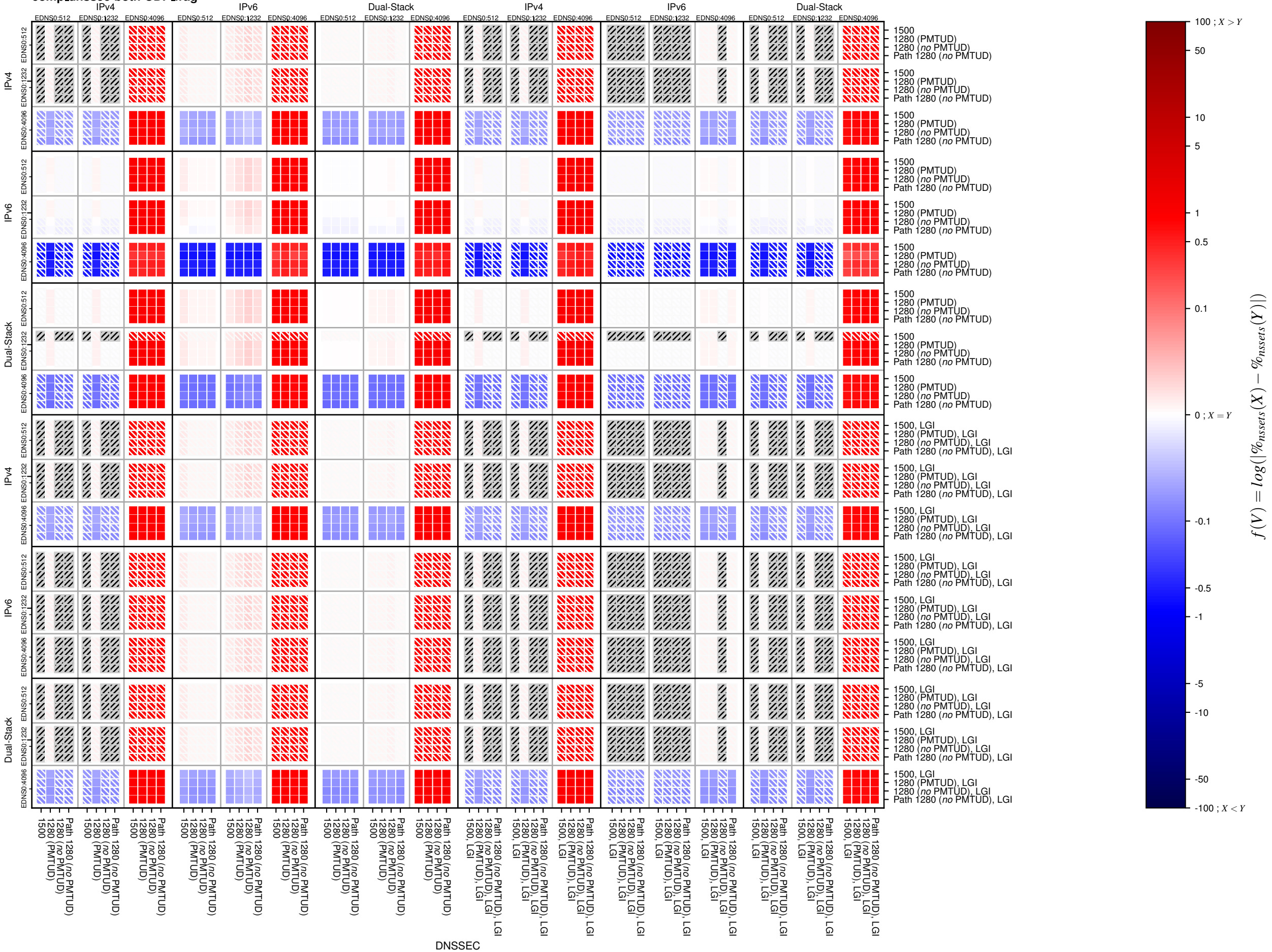
comp_dnssec-both-UDP_frag
