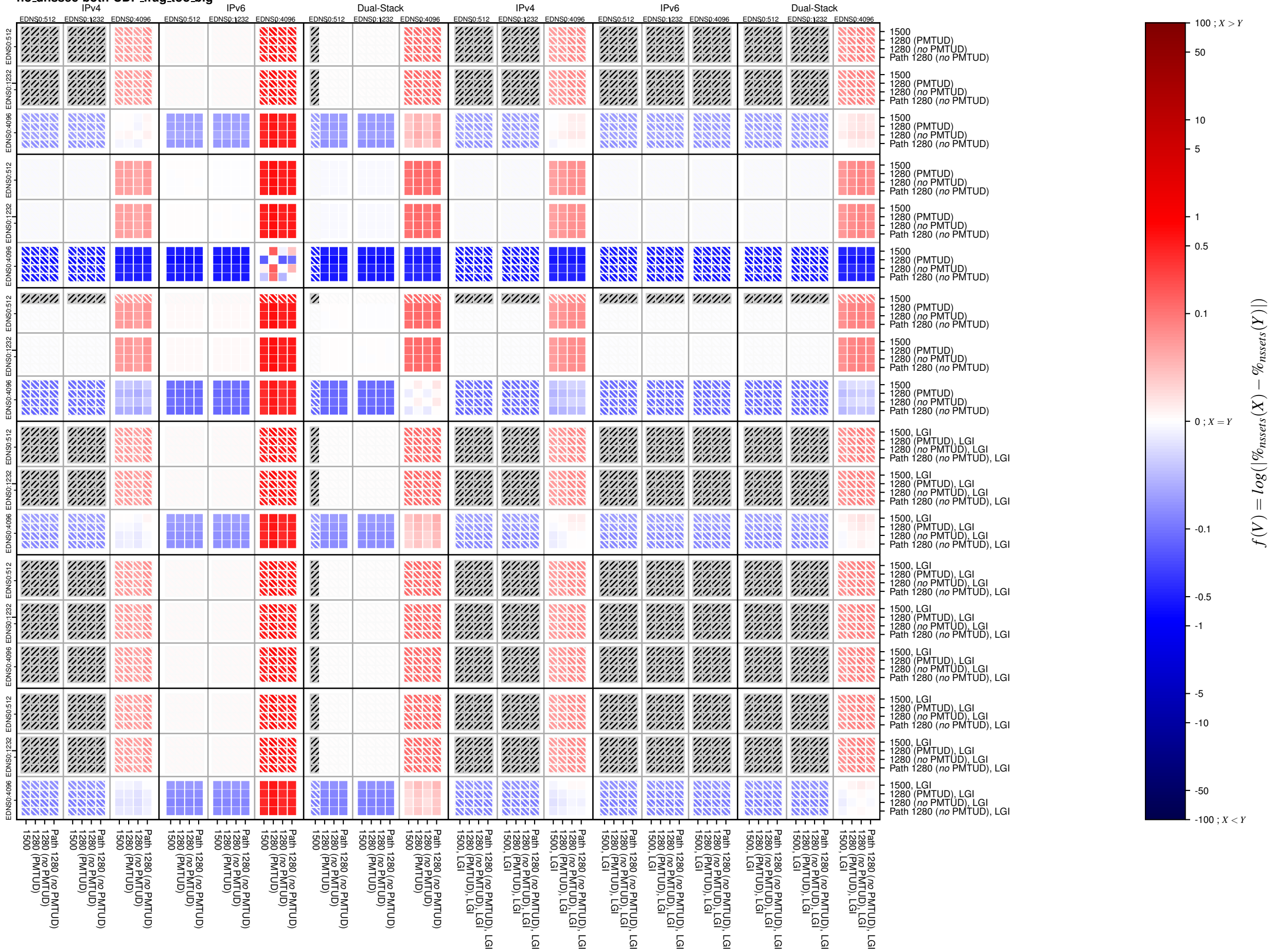
no_dnssec-both-UDP_frag_too_big
