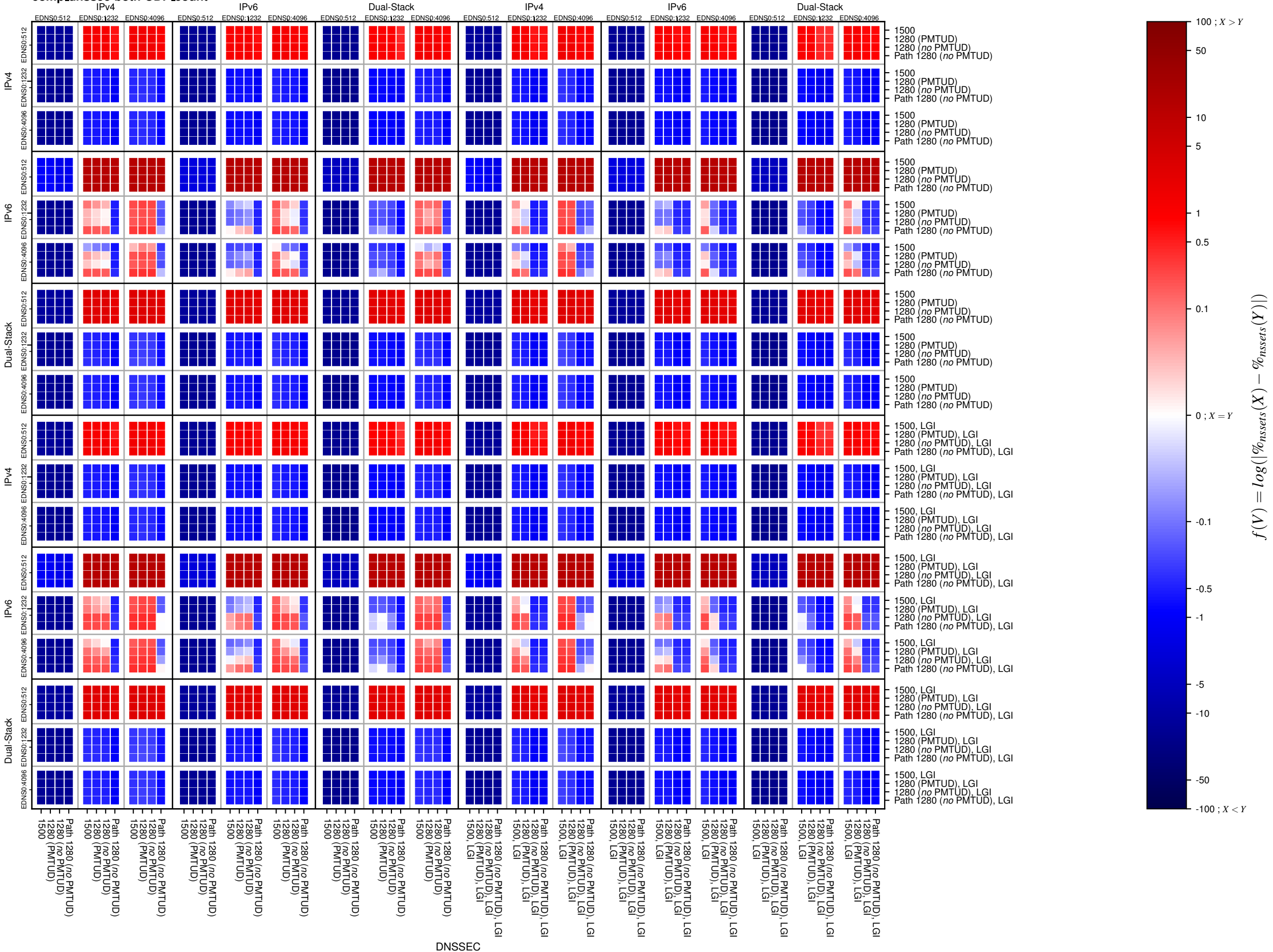
comp_dnssec-both-UDP_count
