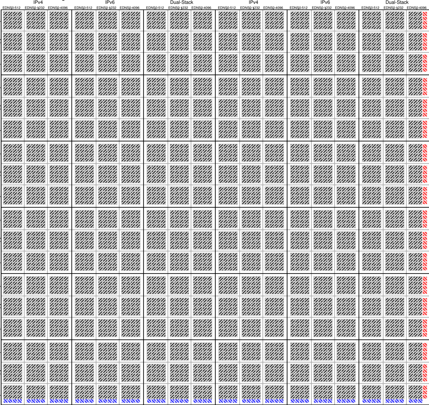
dnssec-both-TCP_frag
