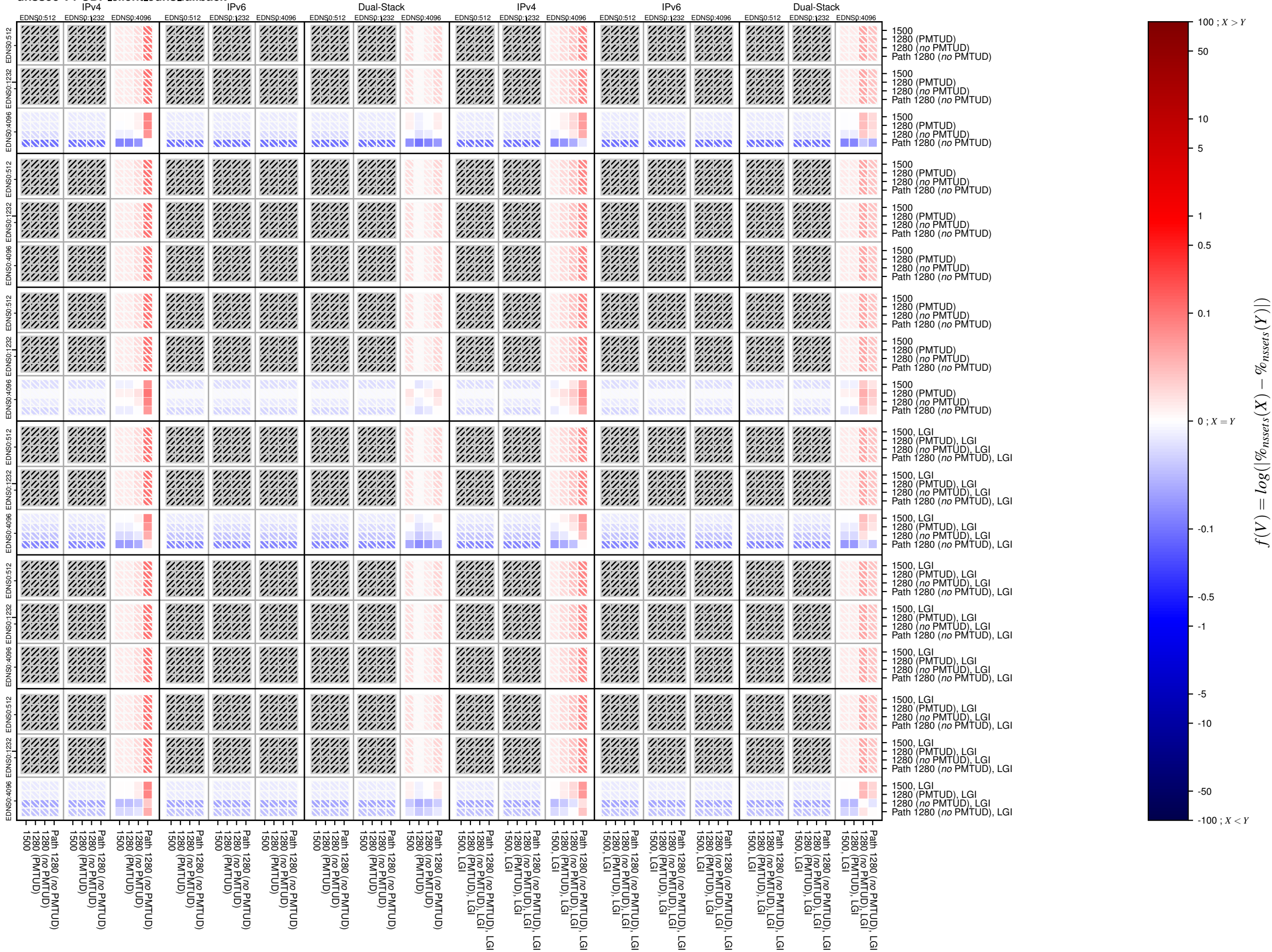
dnssec-v4-UDP_client_edns_fallback
