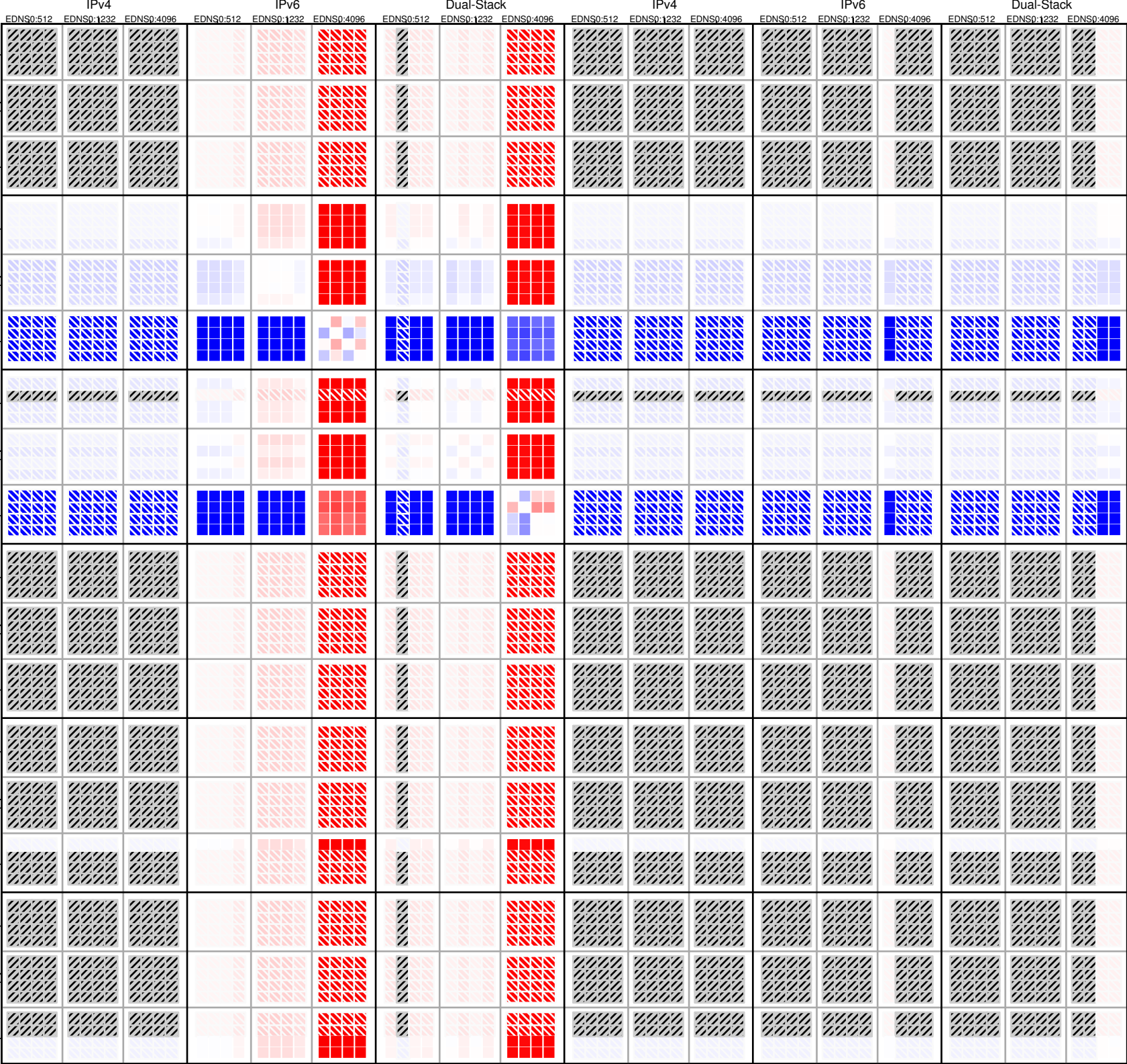
dnssec-v6-UDP_frag.too.big
