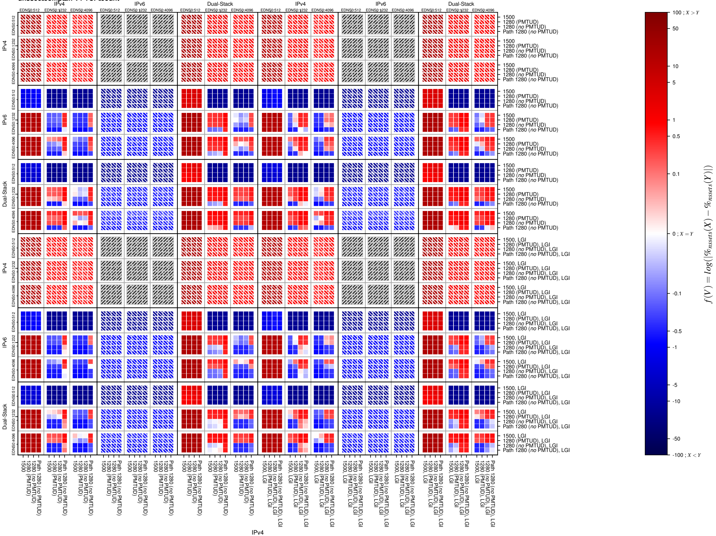
dnssec_comp_afv4-TCP_count
