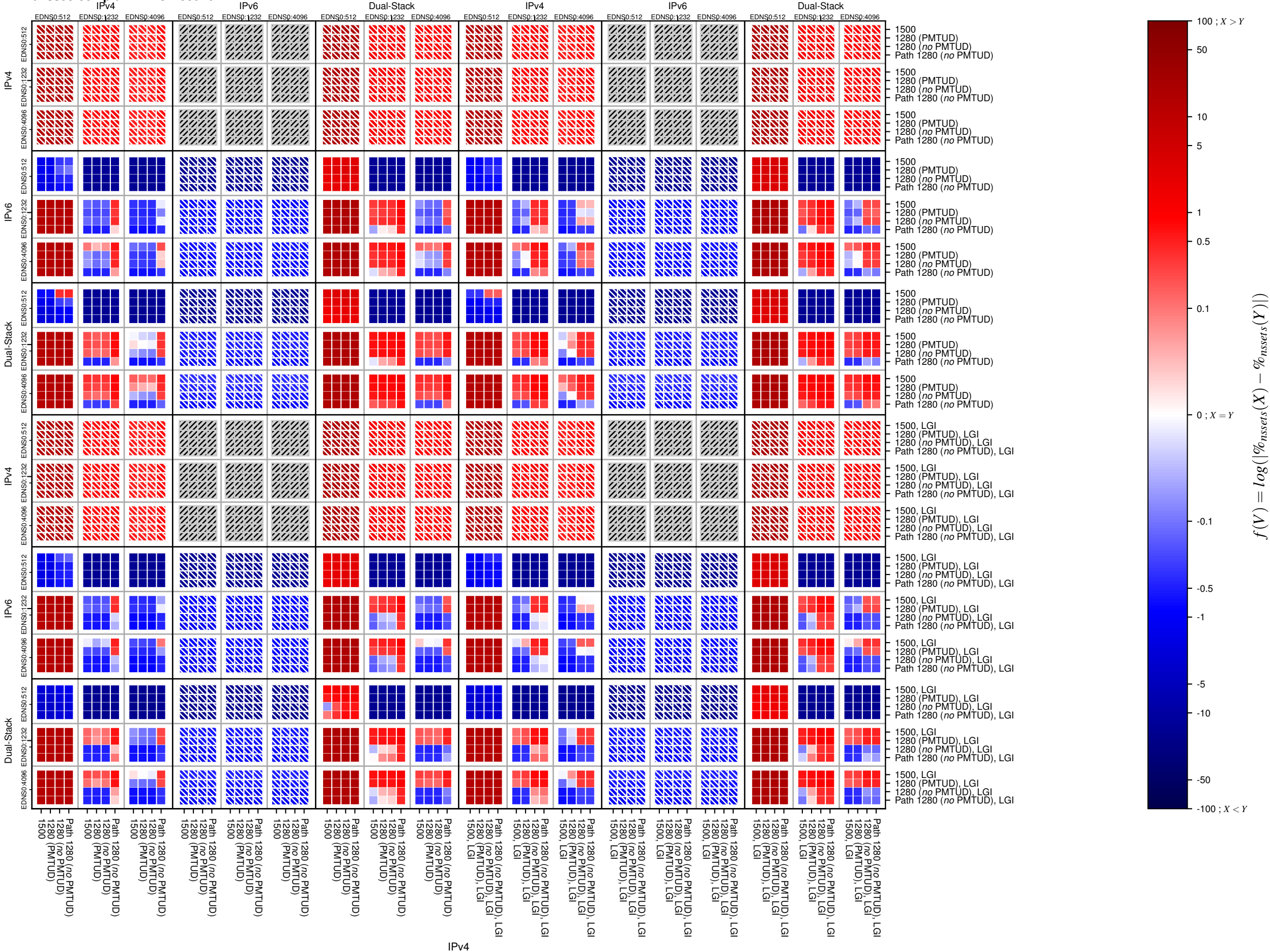
dnssec_comp_afi-v4-TCP_count
