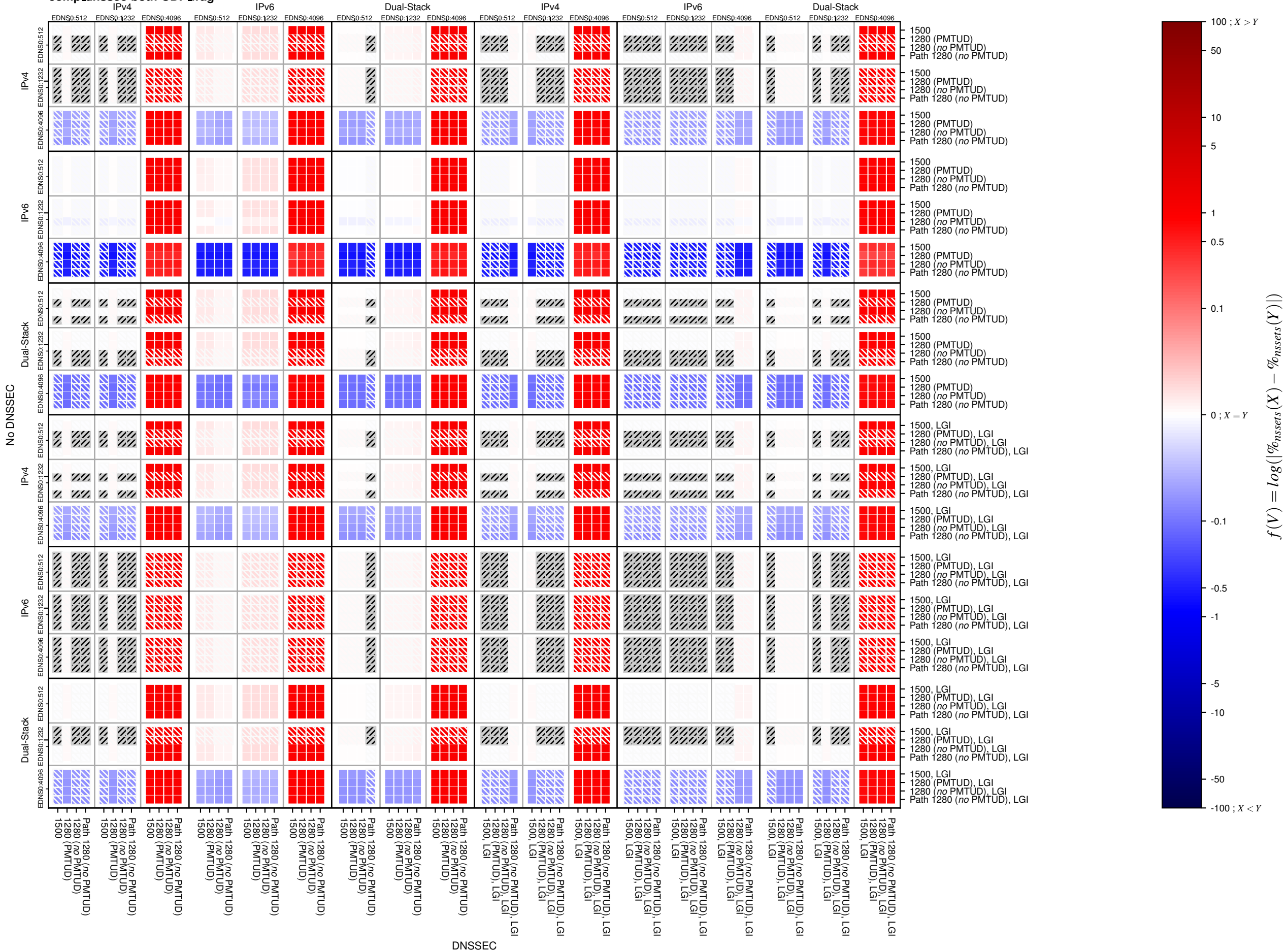
comp_dnssec-both-UDP_frag
