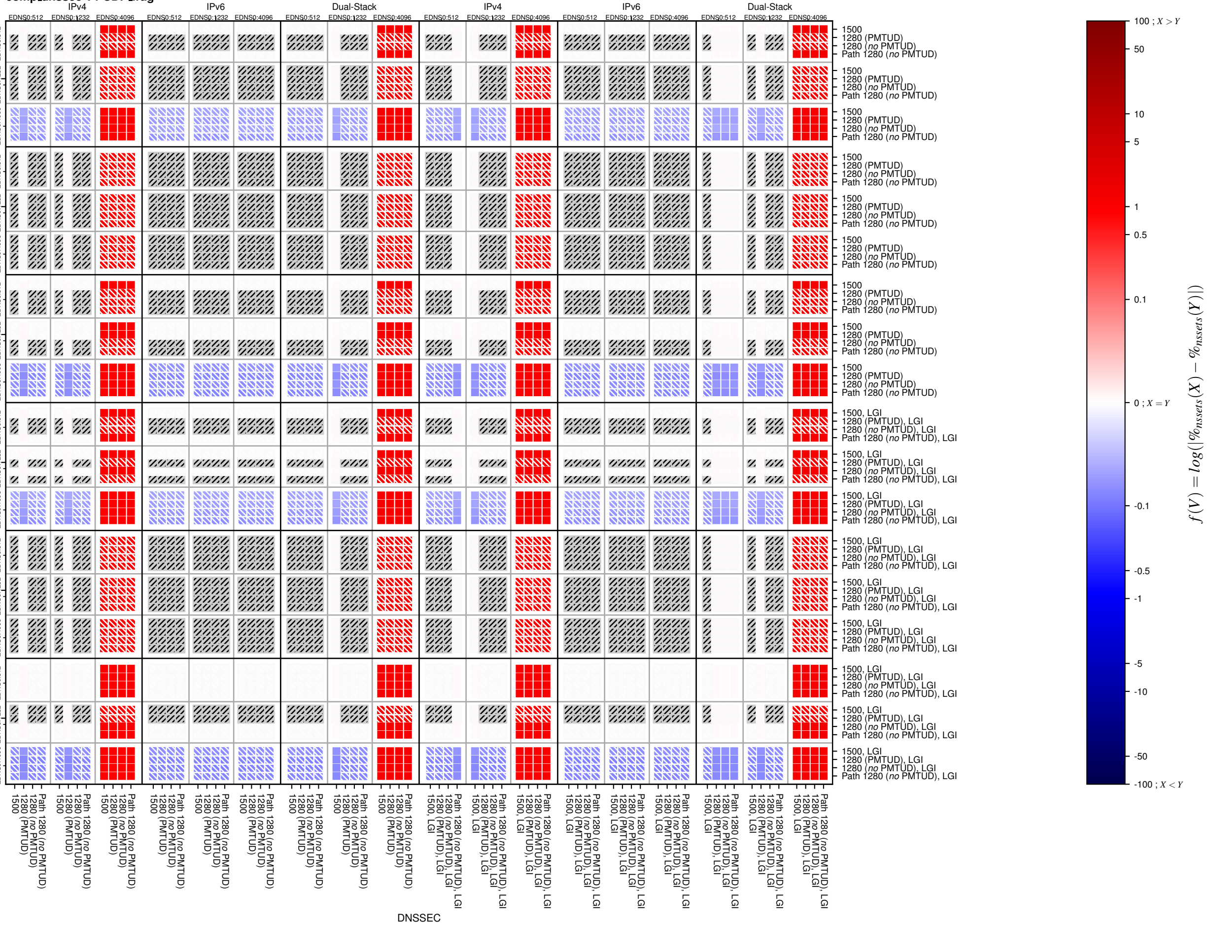
comp_dnssec-v4-UDP_frag
