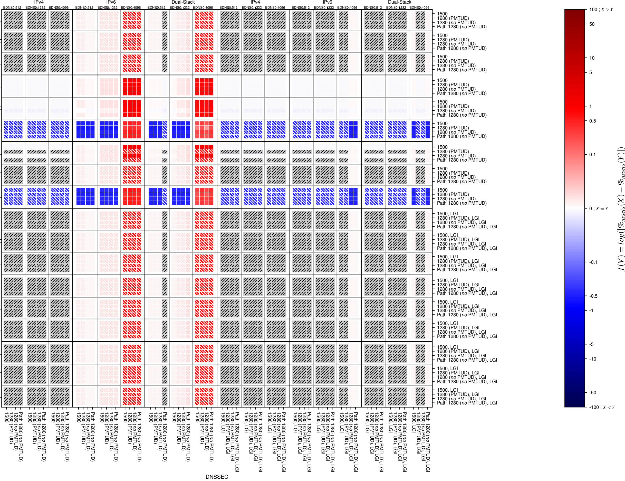
comp_dnssec-v6-UDP_frag_too_big
