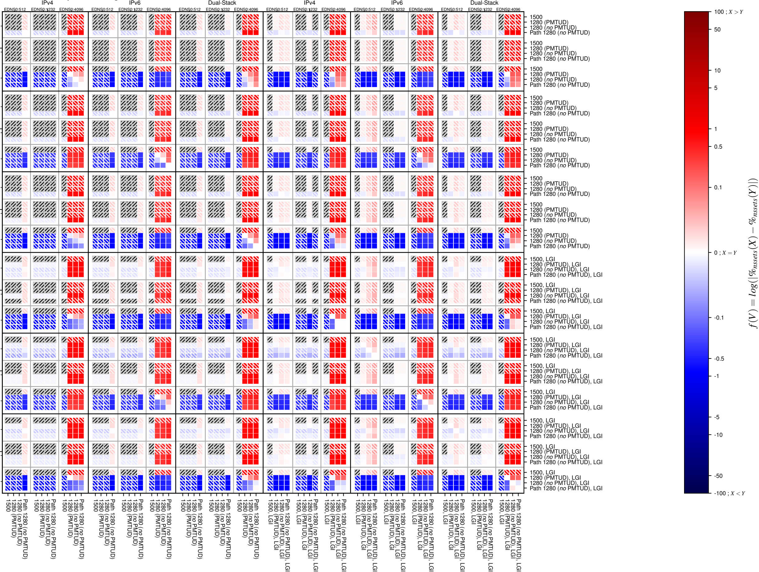
dnssec-both-UDP_packet_too_big
