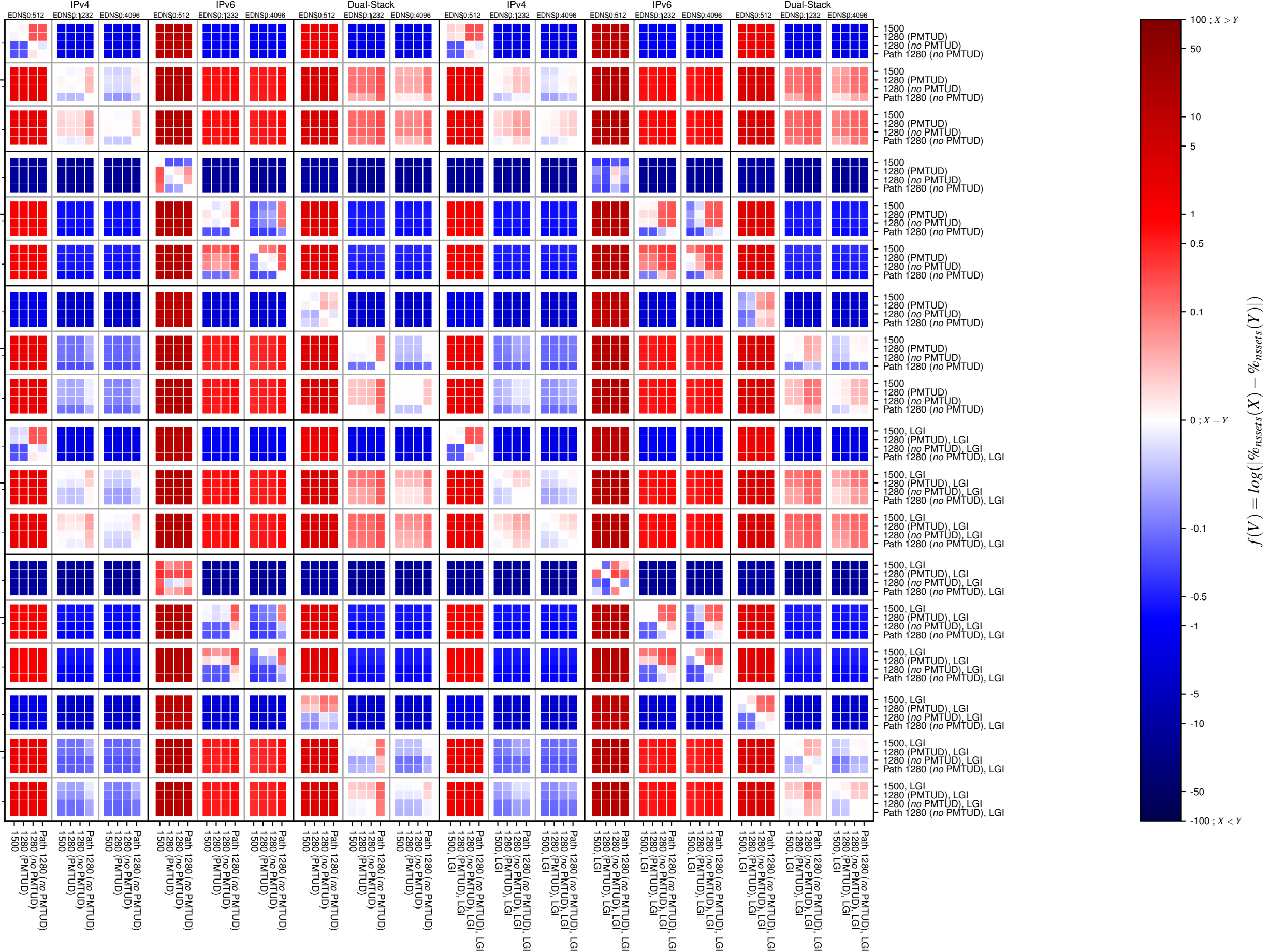
no_dnssec-both-TCP_count
