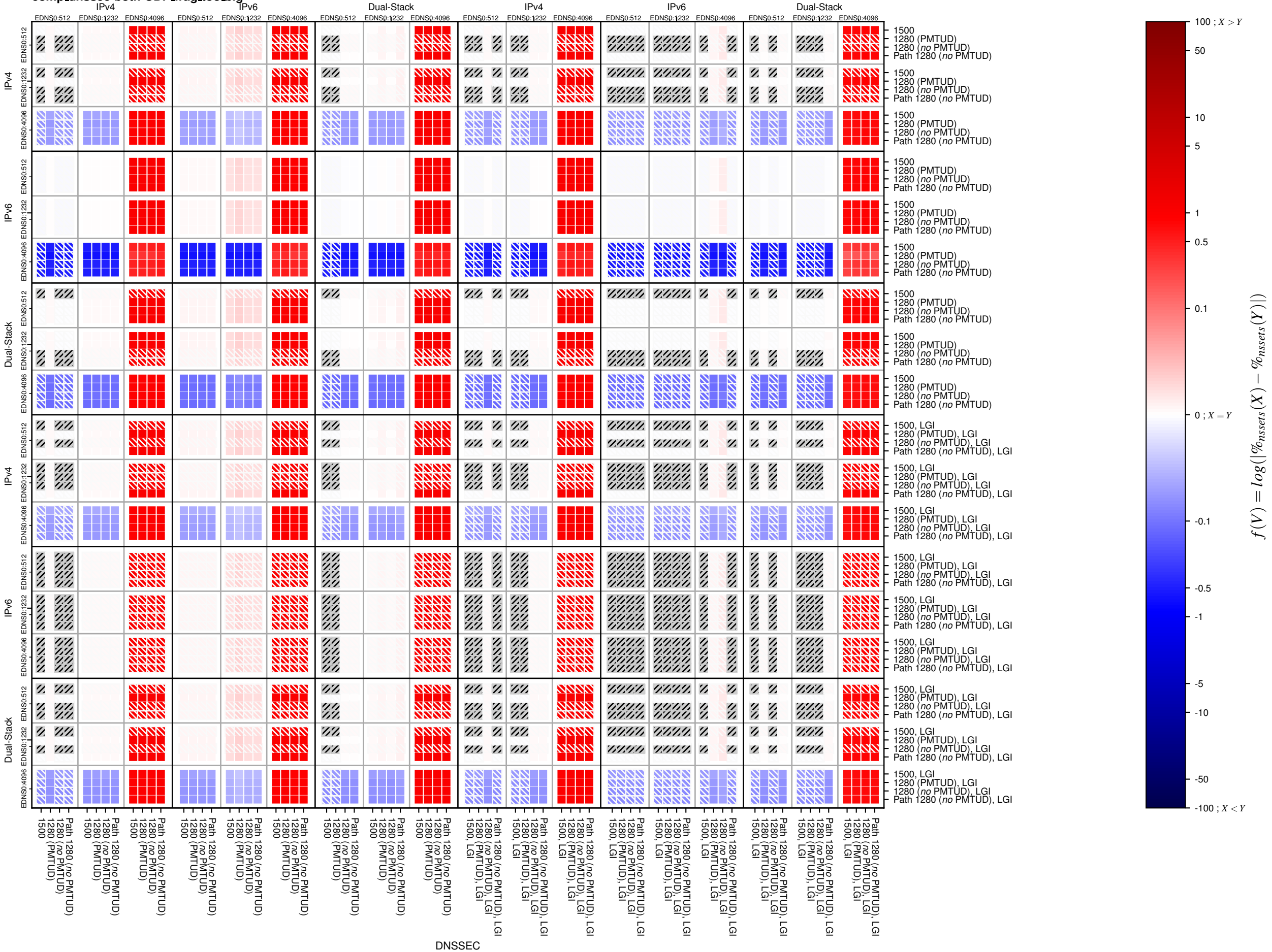
comp_dnssec-both-UDP_frag_too_big
