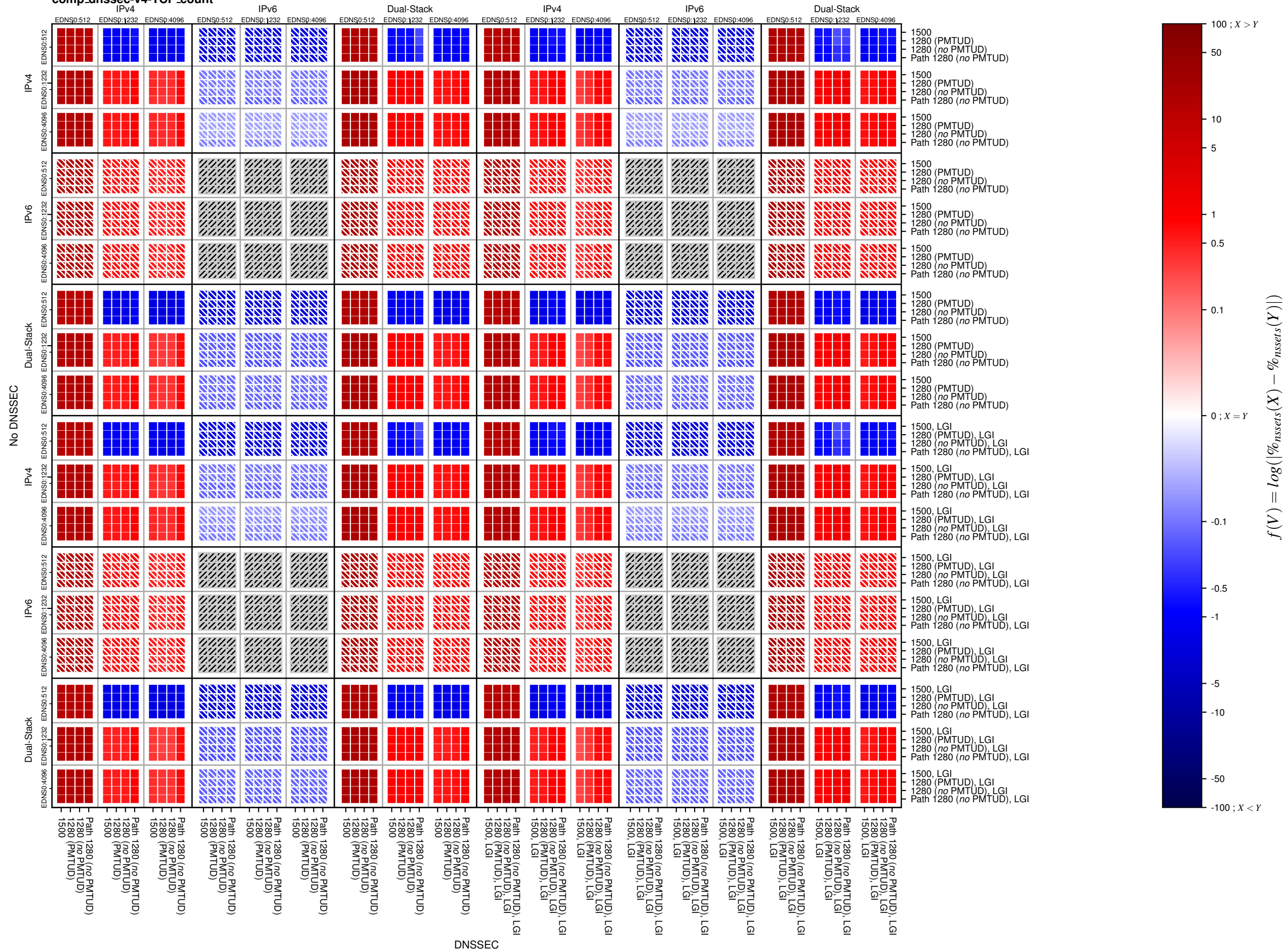
comp_dnssec-v4-TCP_count
