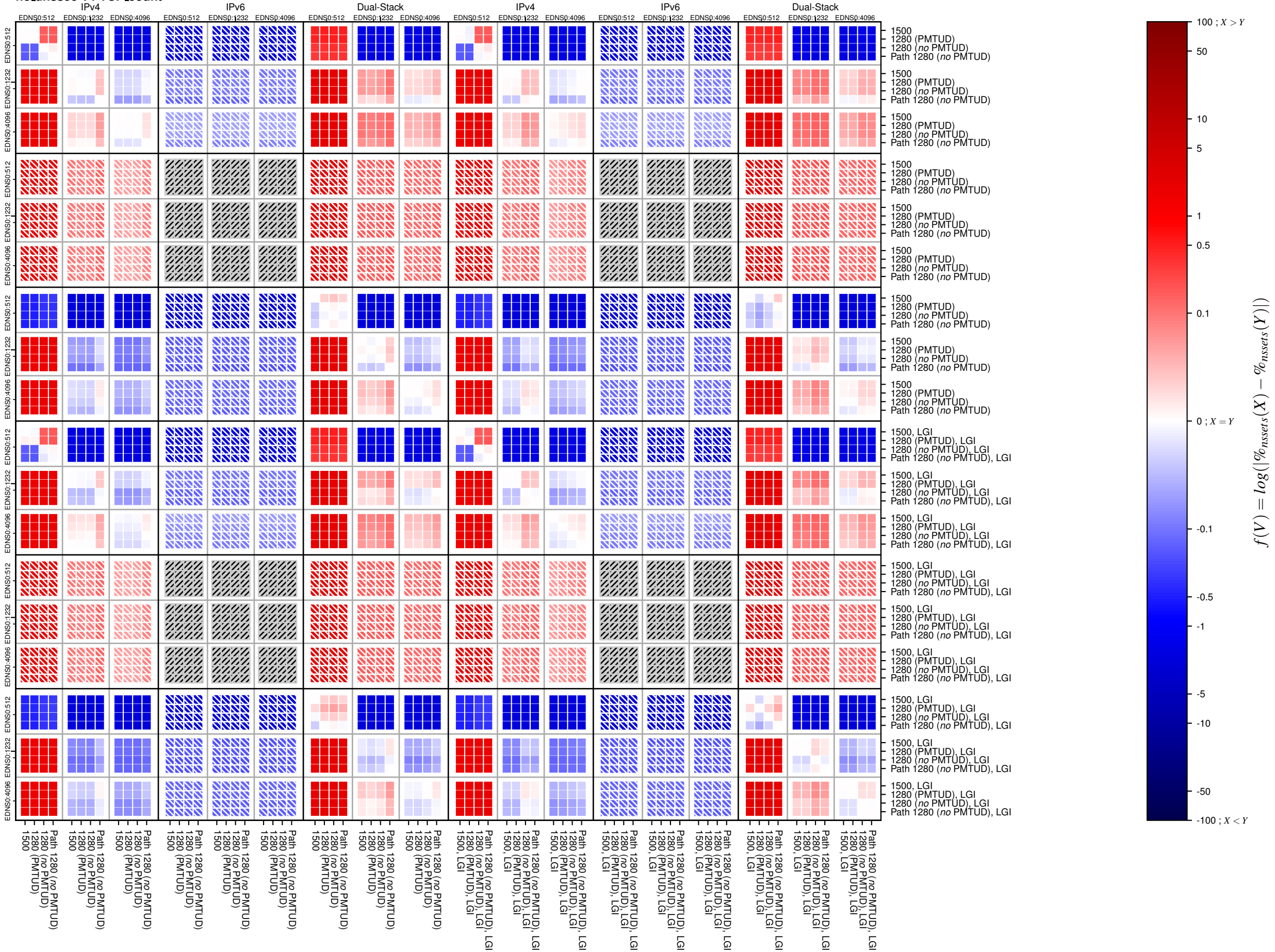
no_dnssec-v4-TCP_count
