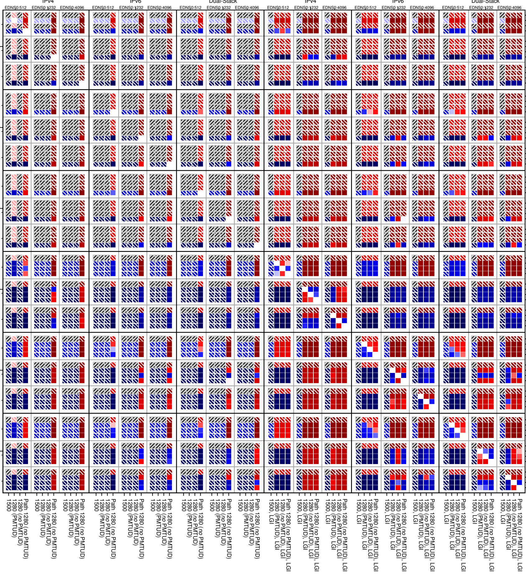
dnssec-both-TCP_packet_too_big
