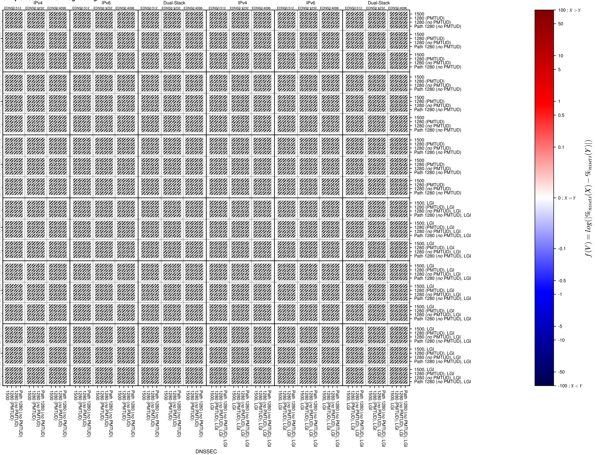
comp_dnssec-v4-TCP_frag_too_big
