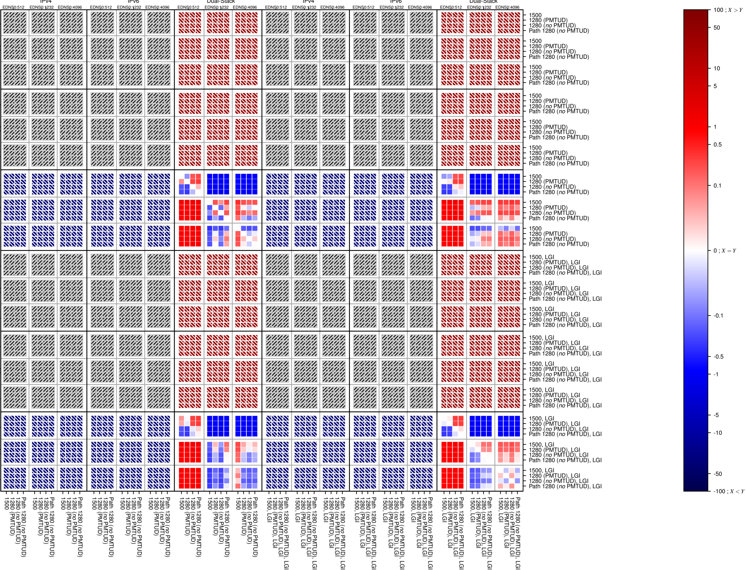
dnssec-v6-UDP_TCP_afi_count
