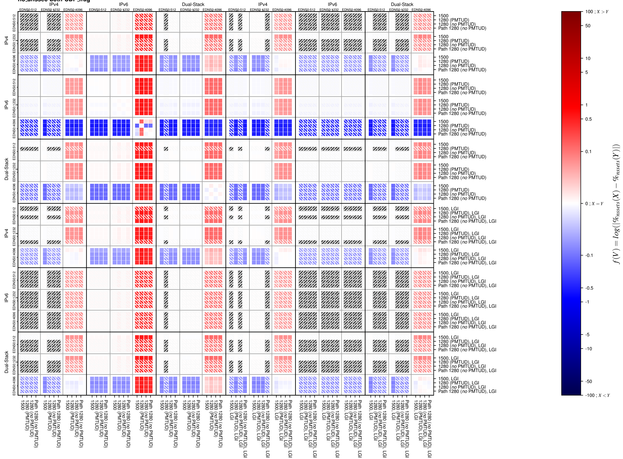
no_dnssec-both-UDP_frag
