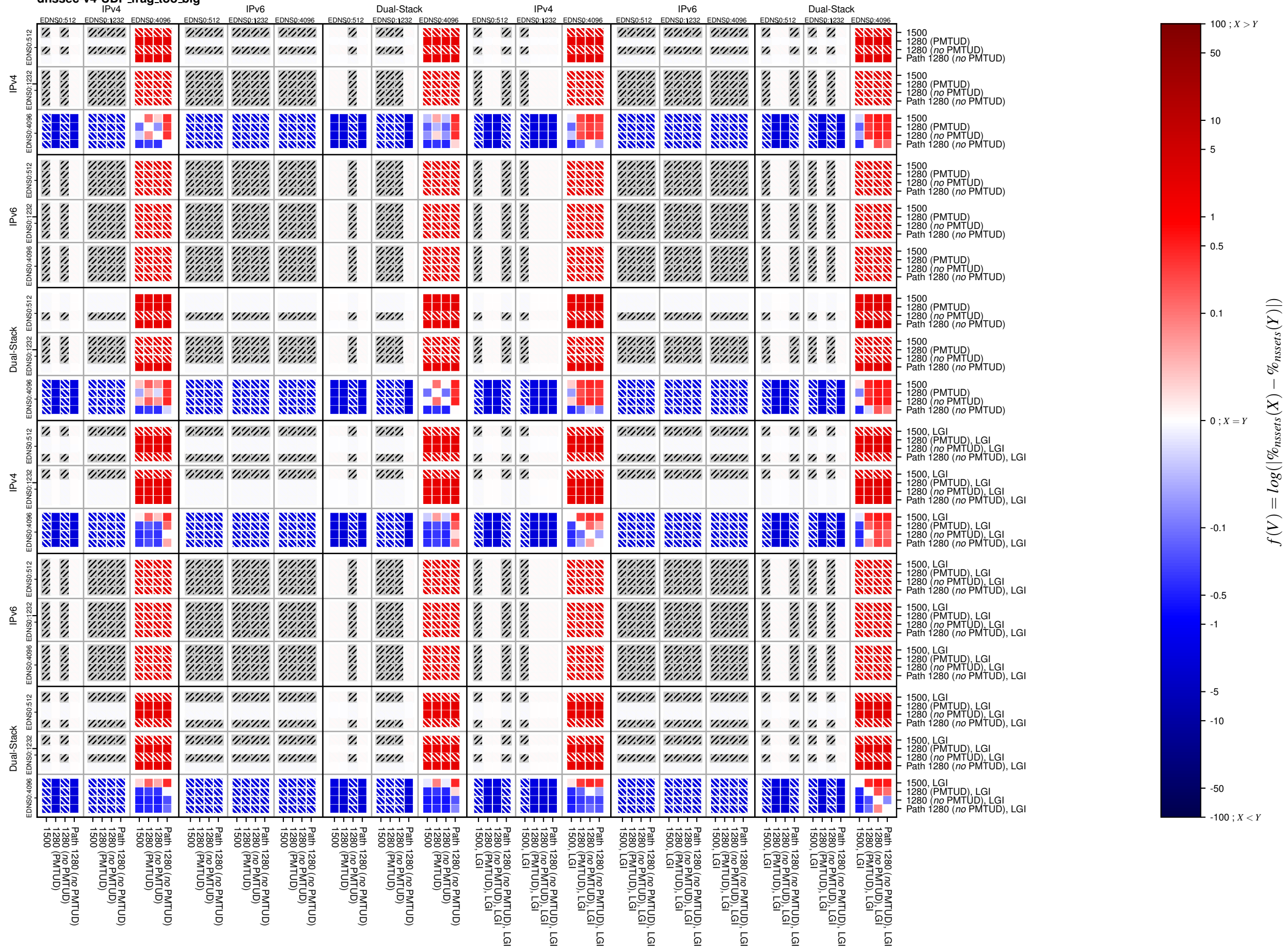
dnssec-v4-UDP_frag_too_big
