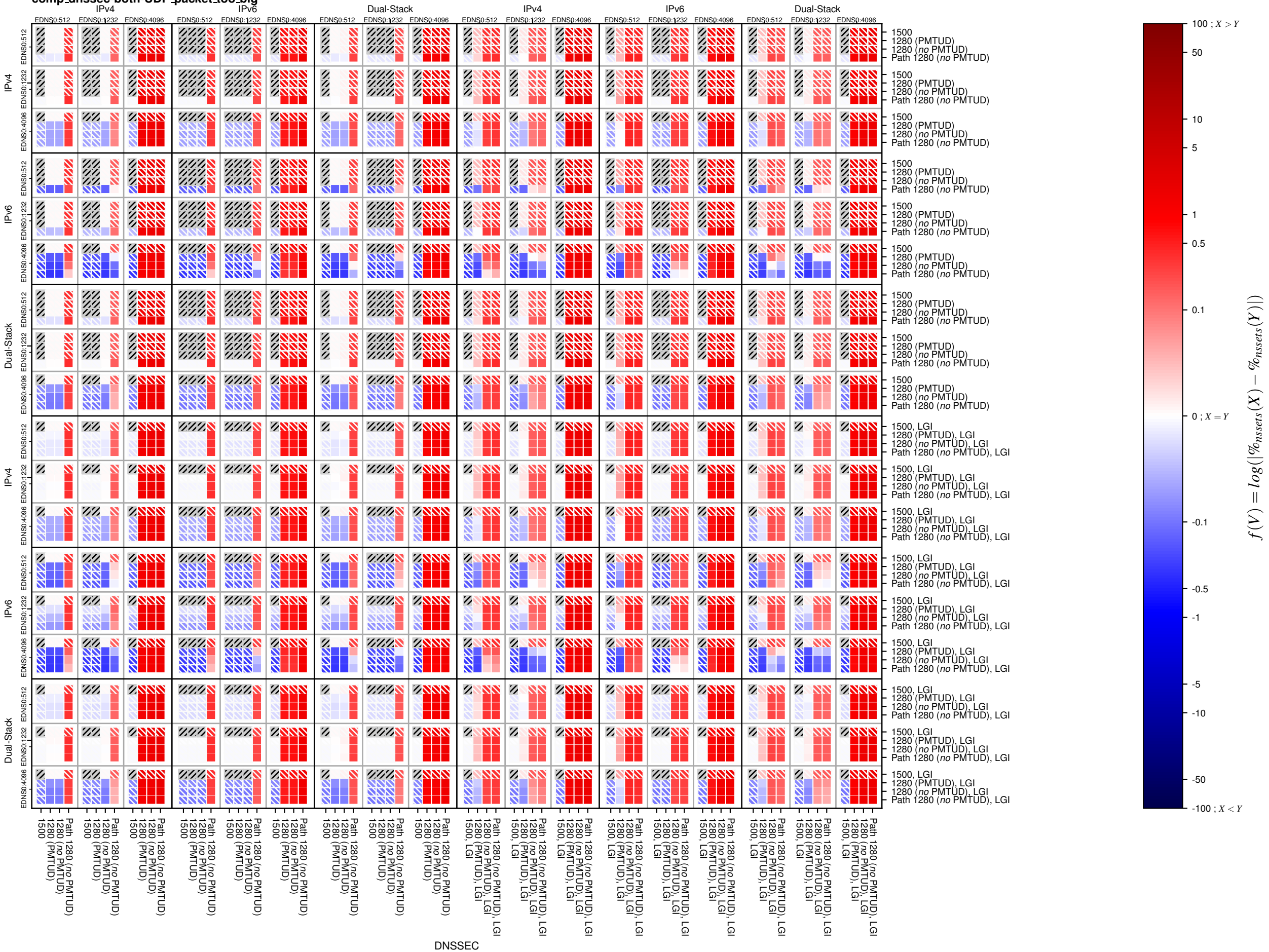
comp_dnsssec-both-UDP_packet_too_big
