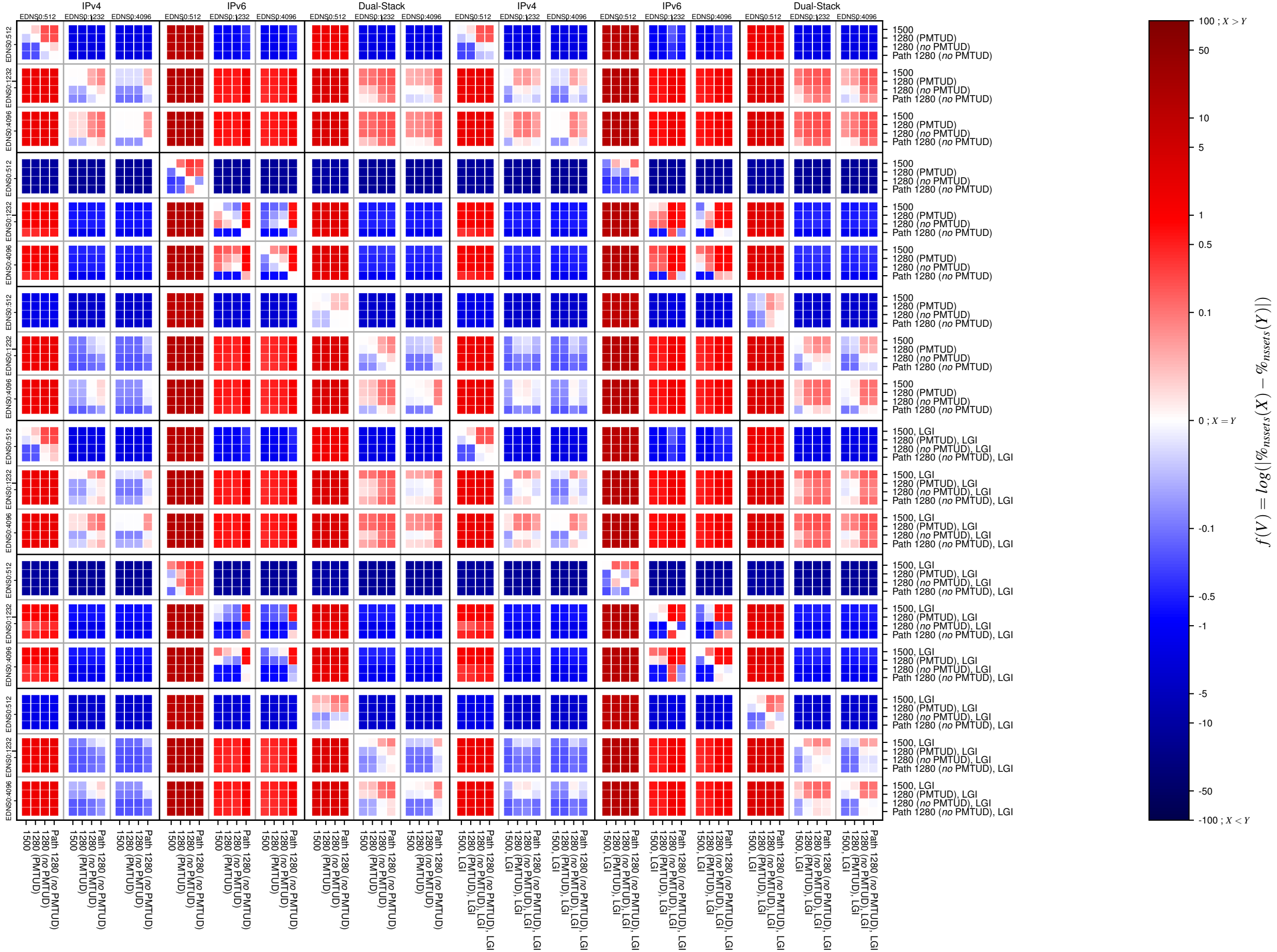
no_dnssec-both-TCP_count
