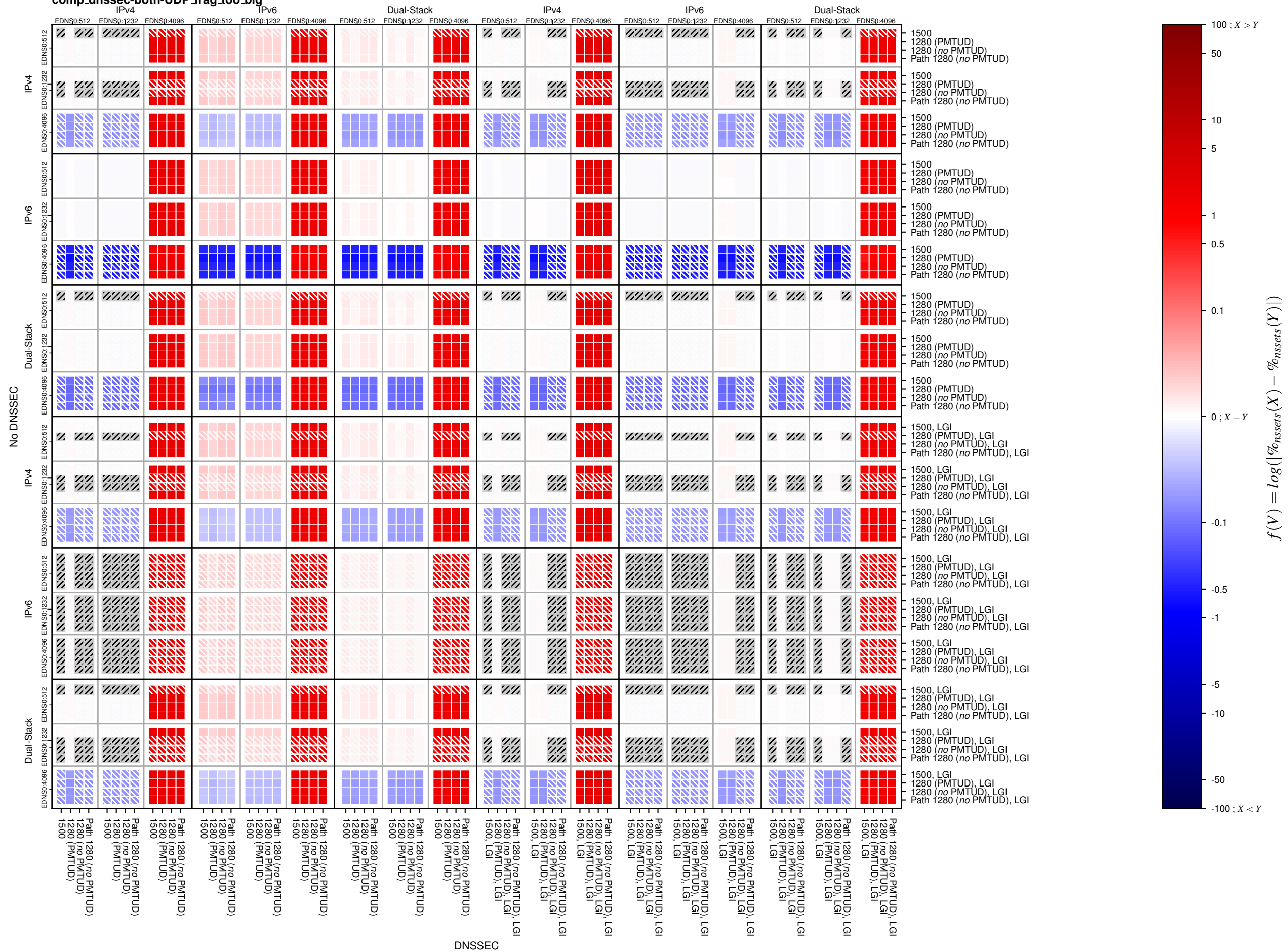
comp_dnsssec-both-UDP_frag_too_big
