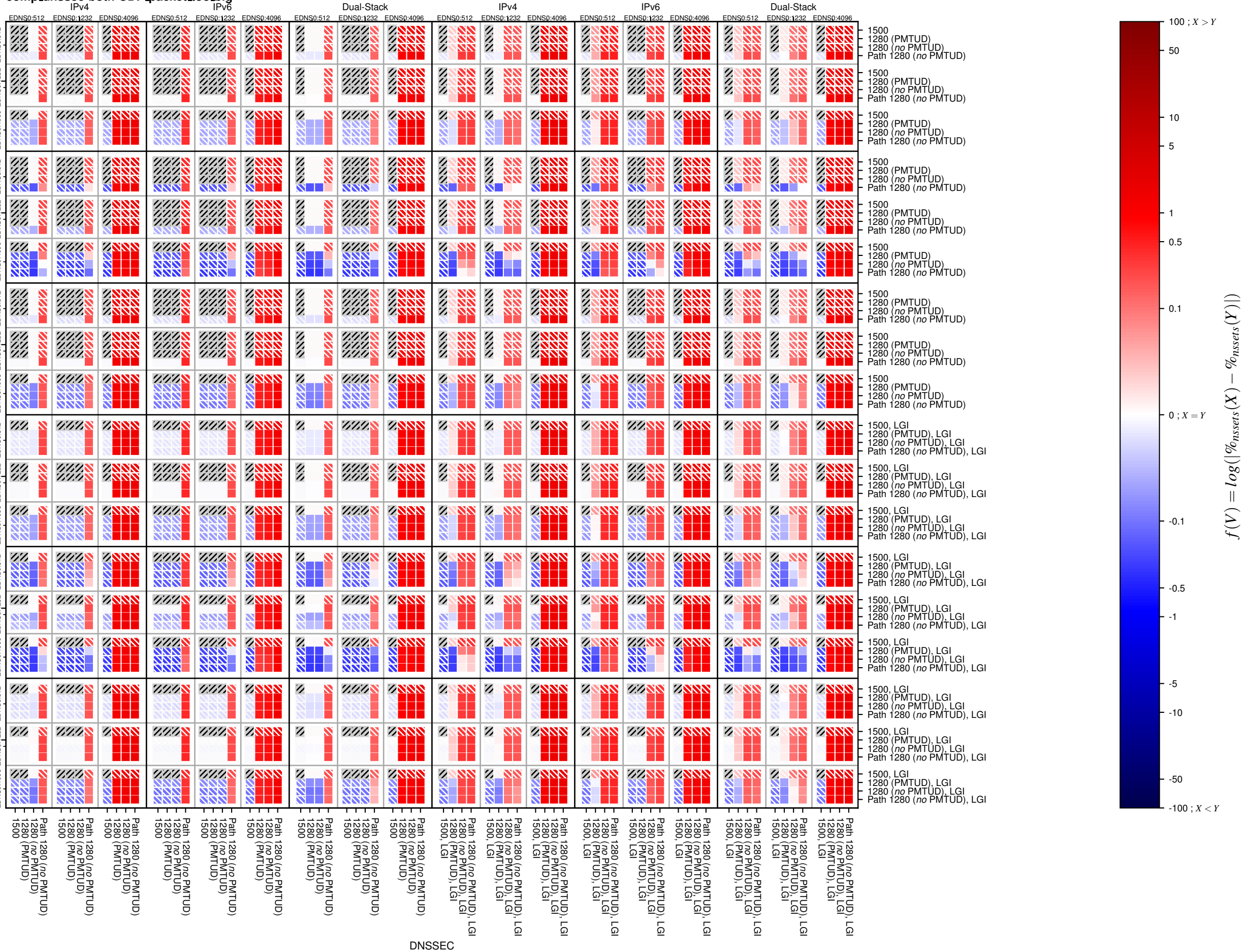
comp_dnsssec-both-UDP_packet_too_big
