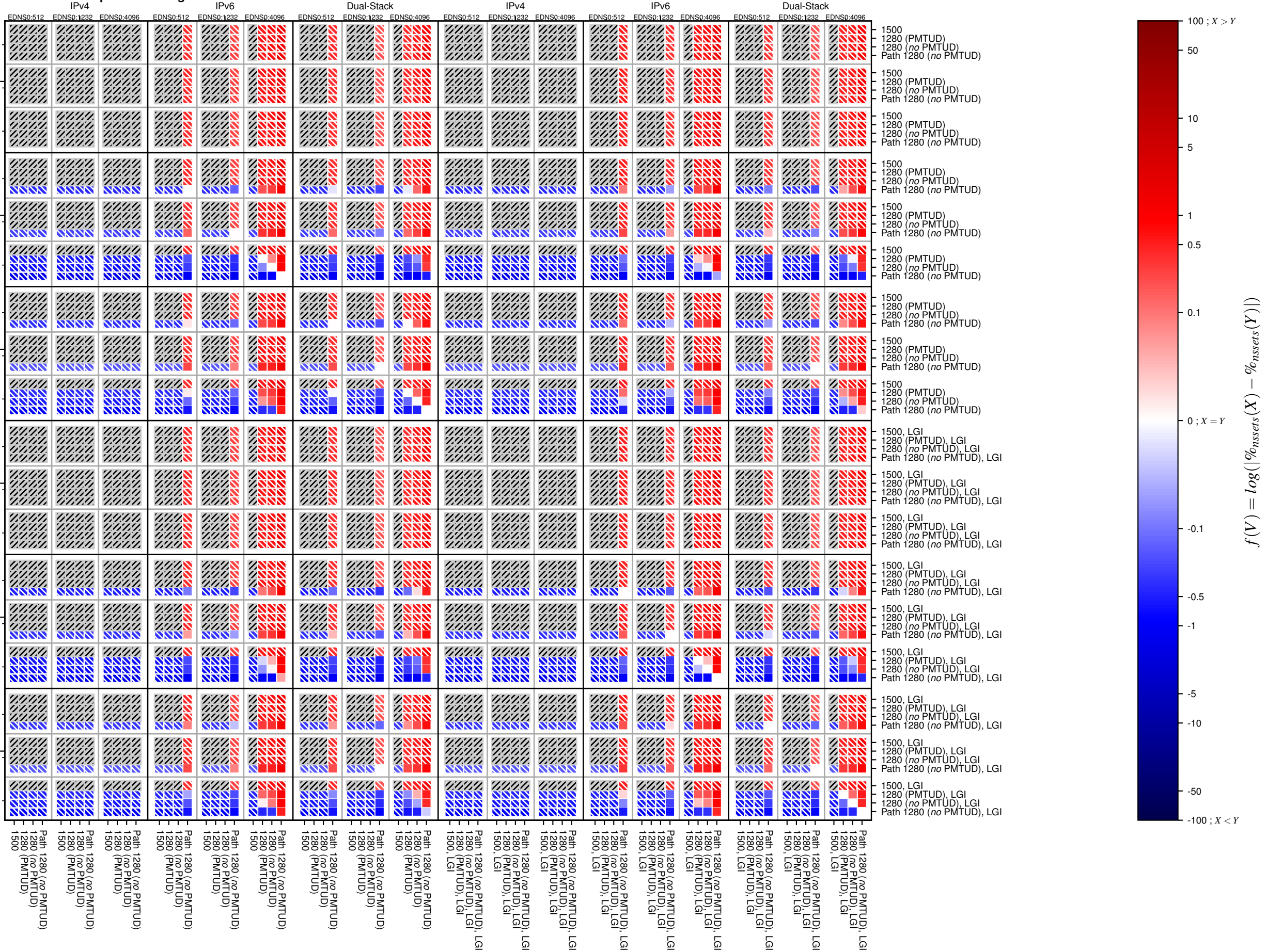
dnssec-v6-UDP_packet_too_big
