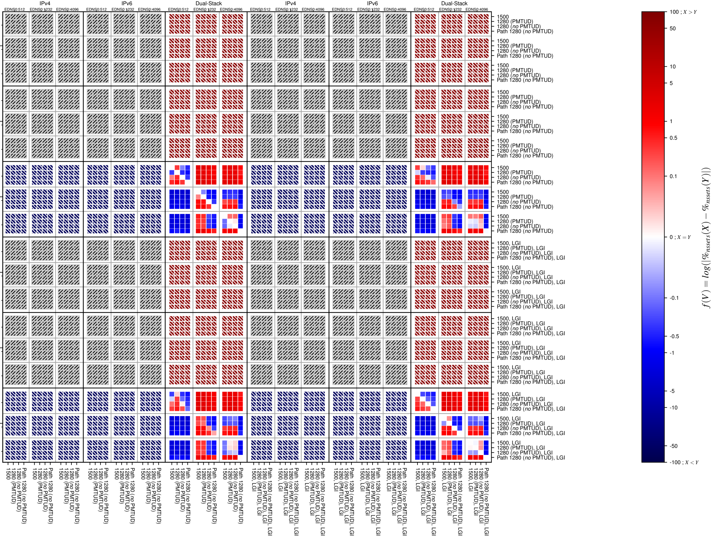
dnssec-v4-UDP_TCP_afc_count
