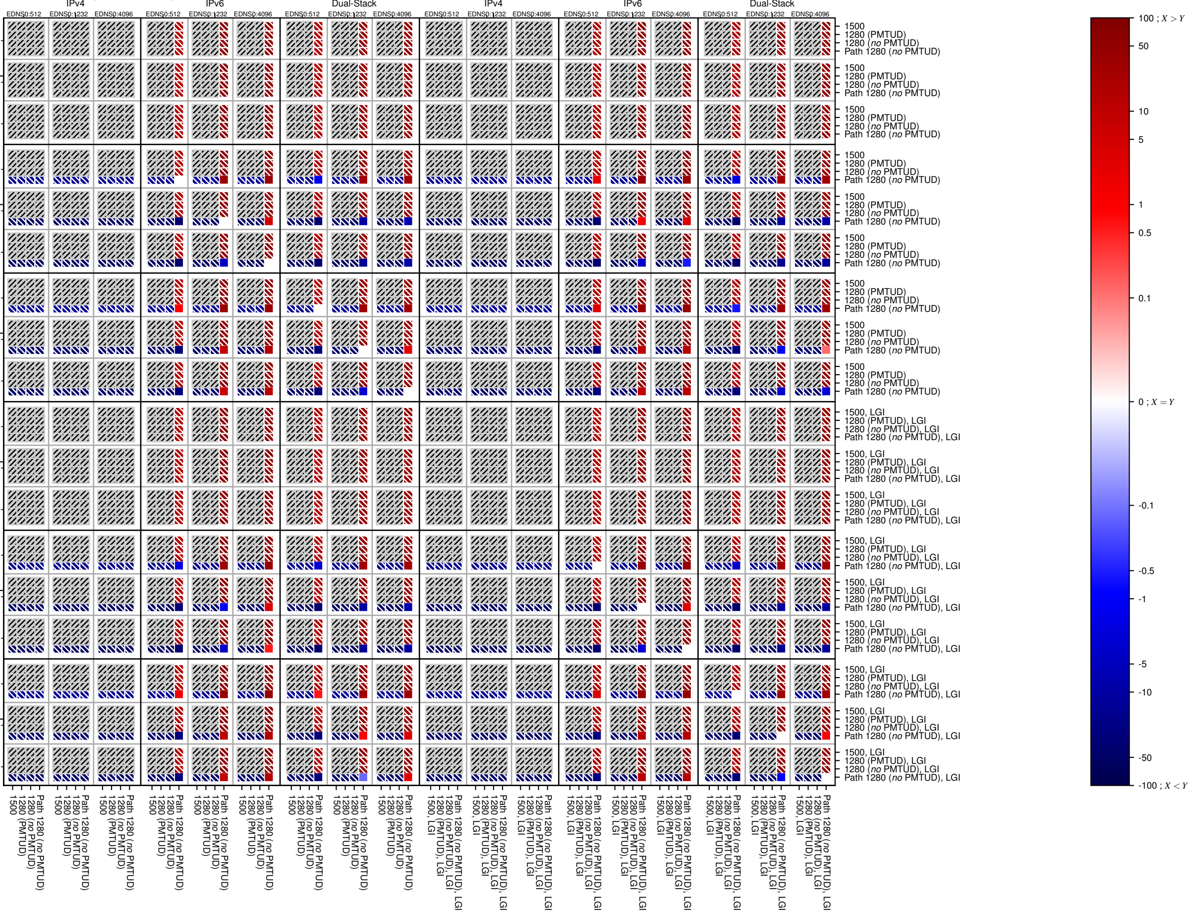
dnssec-v6-TCP_packet_too_big
