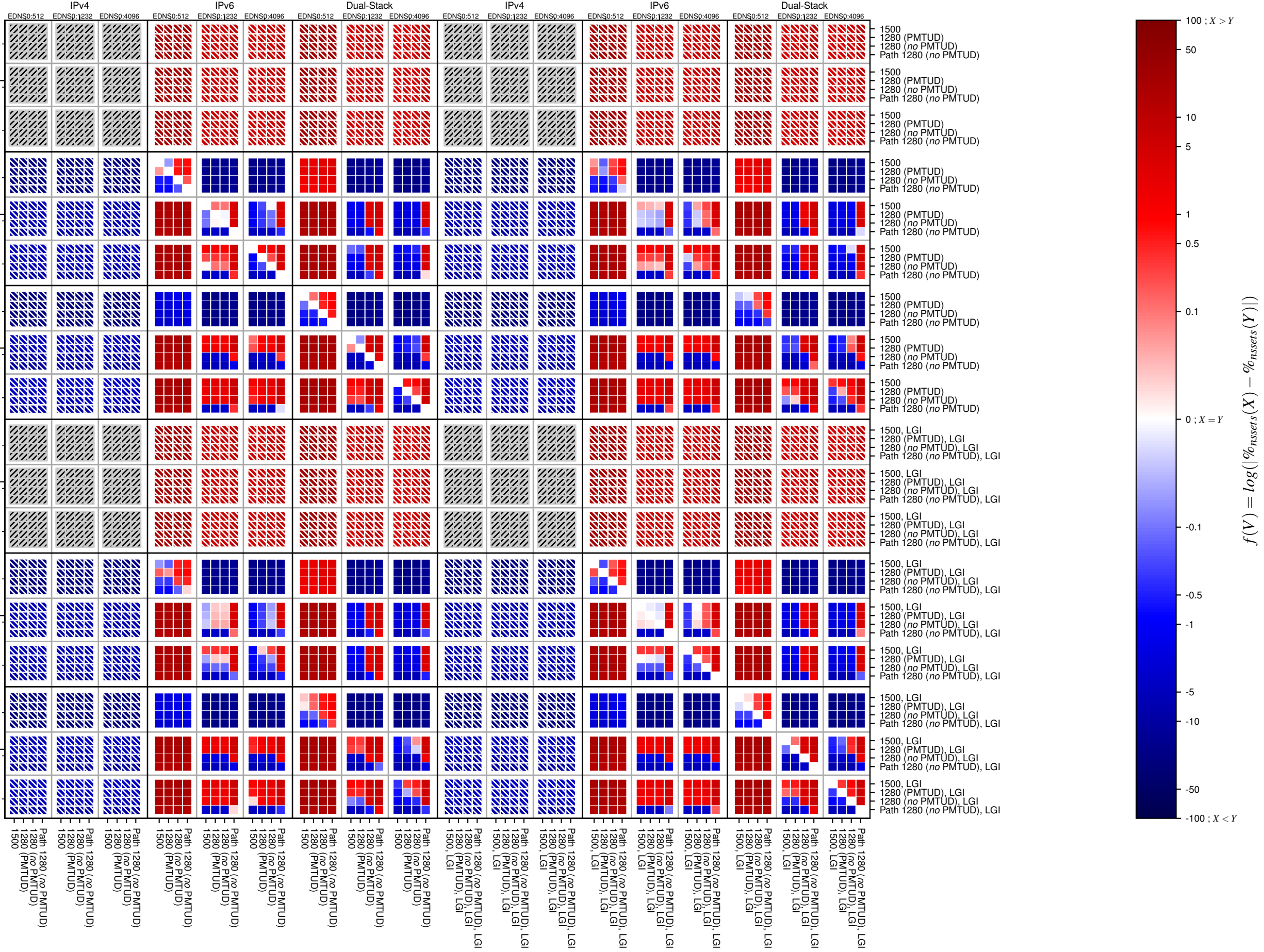
dnssec-v6-TCP_count
