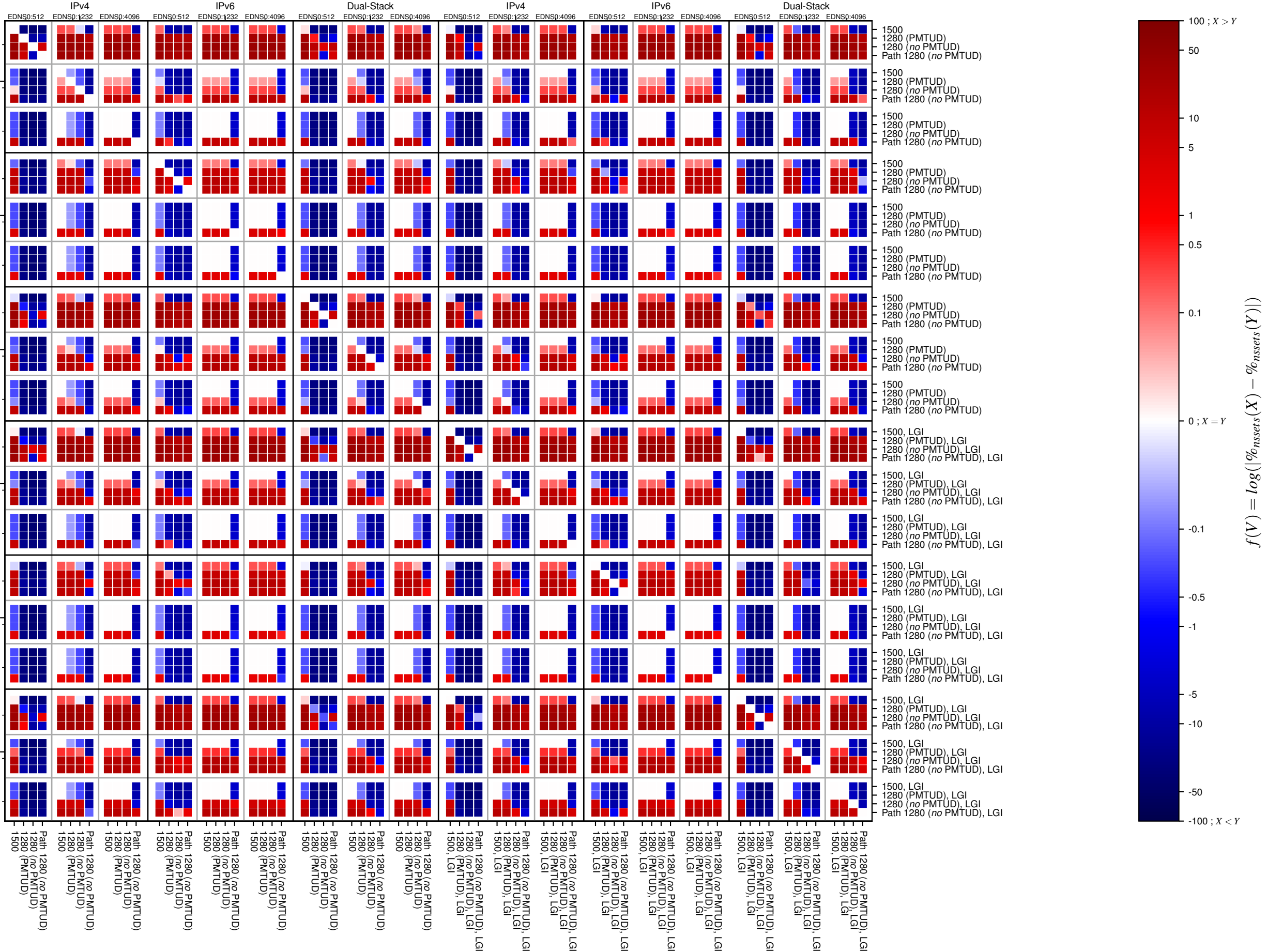
dnssec-both-TCP_server_mss_ok
