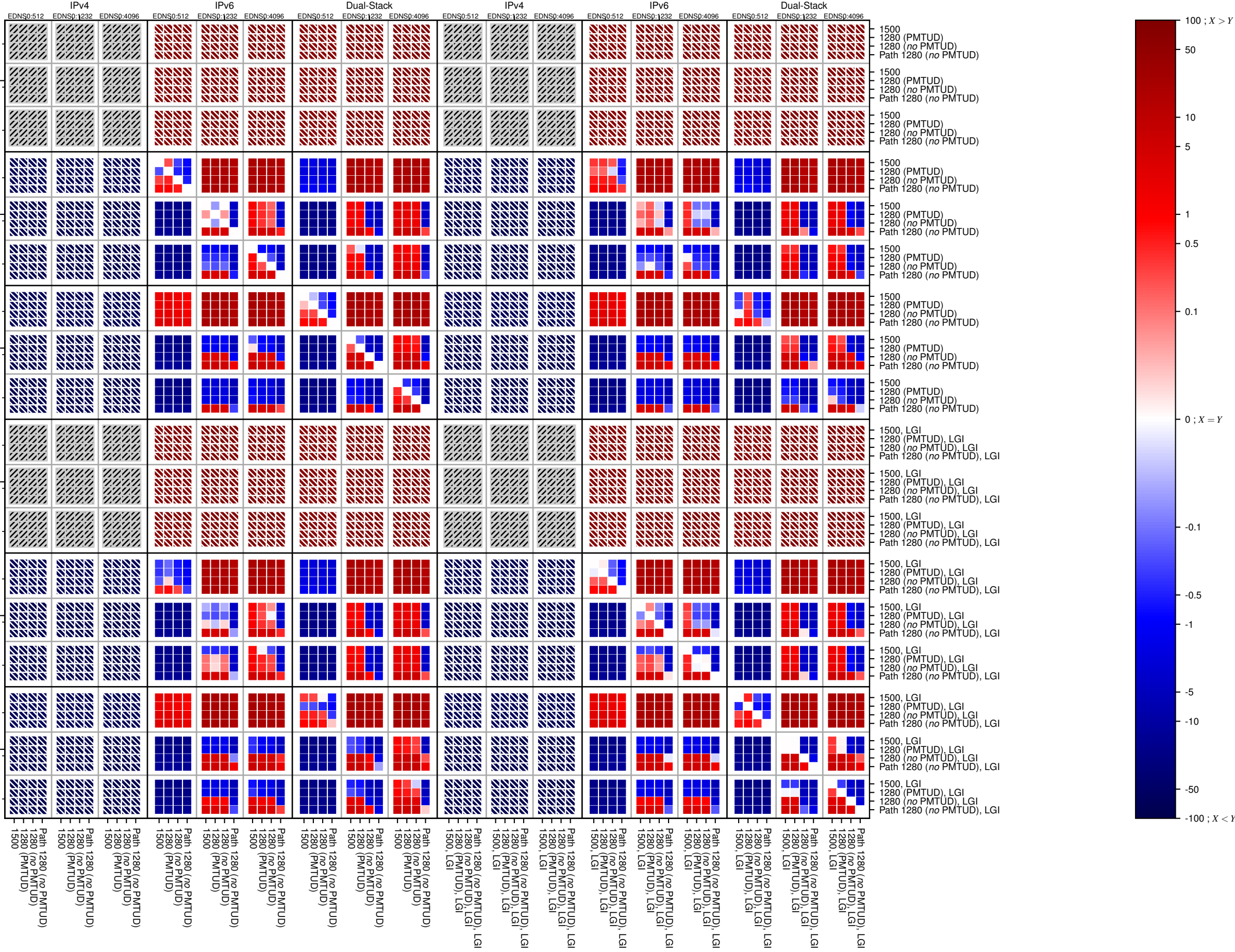
dnssec-v6-UDP_count
