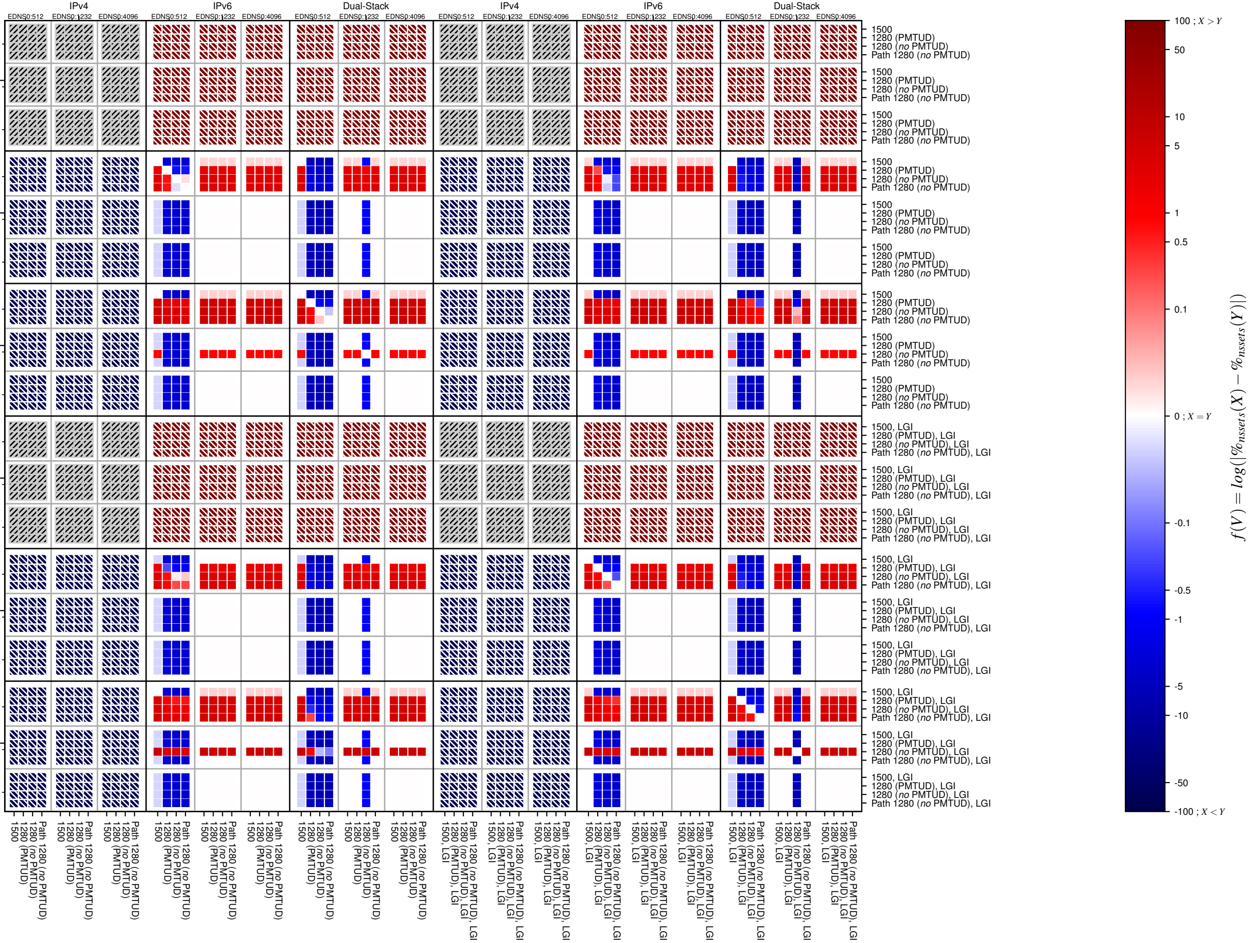
no_dnssec-v6-TCP_server_mss_ok
