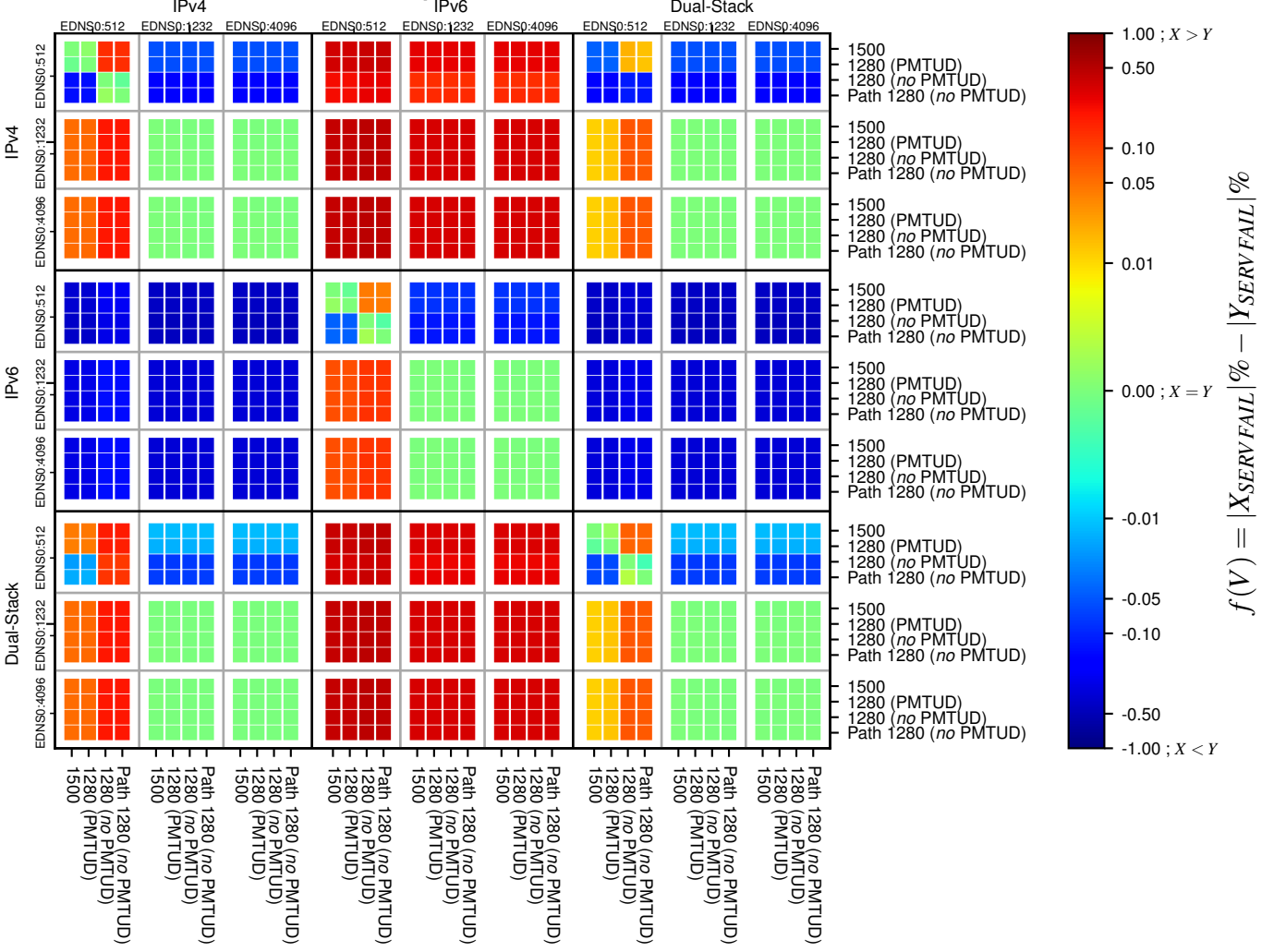
All Zones without DNSSEC for ‘all.psl.domains’
