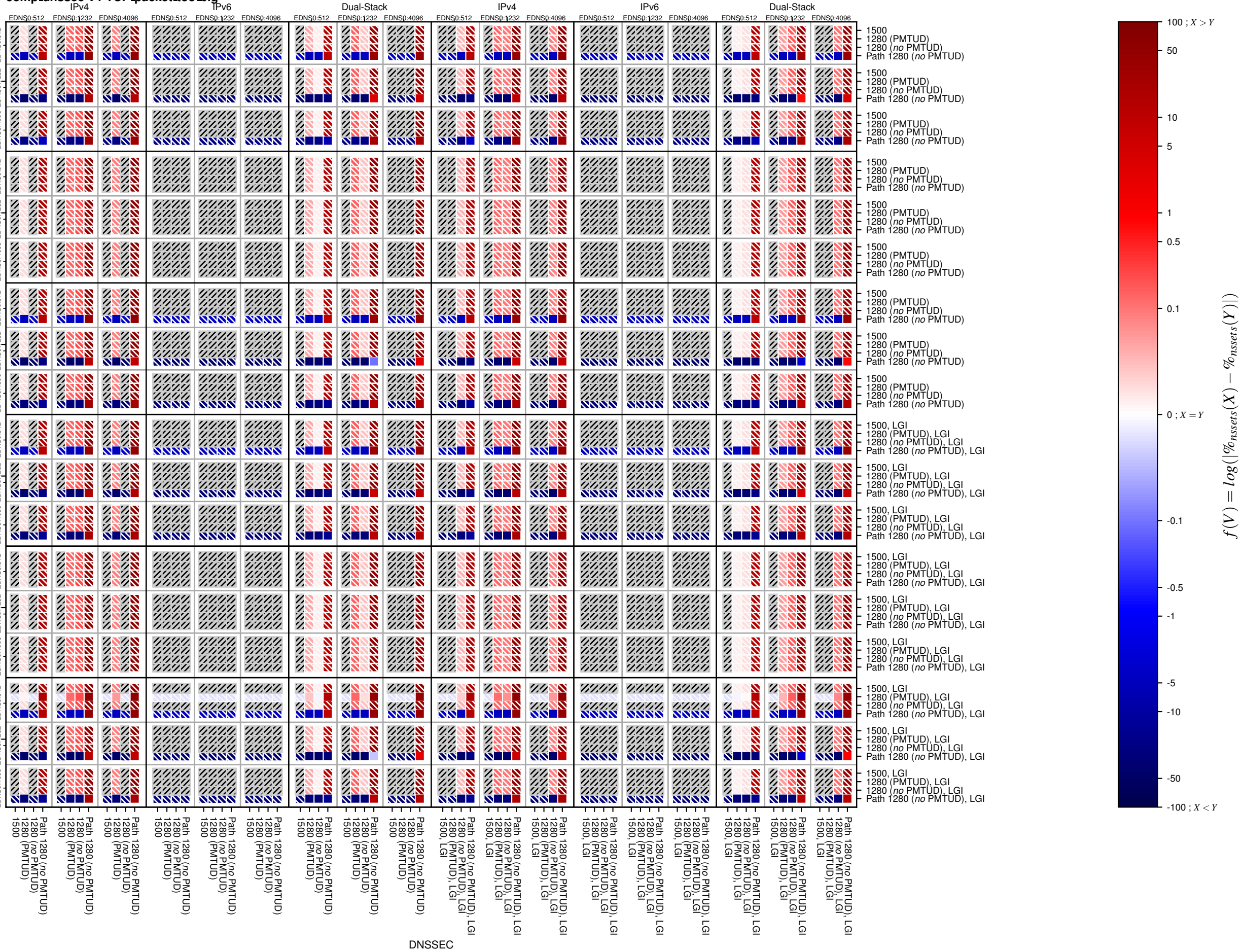
comp_dnssec-v4-TCP_packet_too_big
