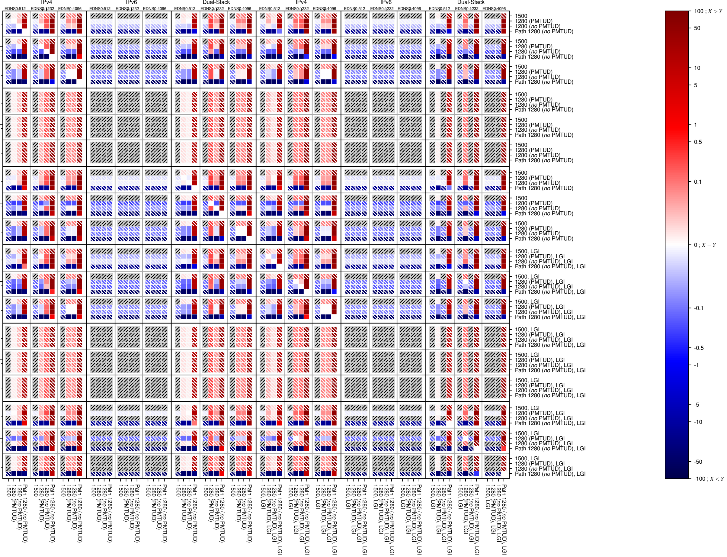
dnssec-v4-TCP_packet_too_big
