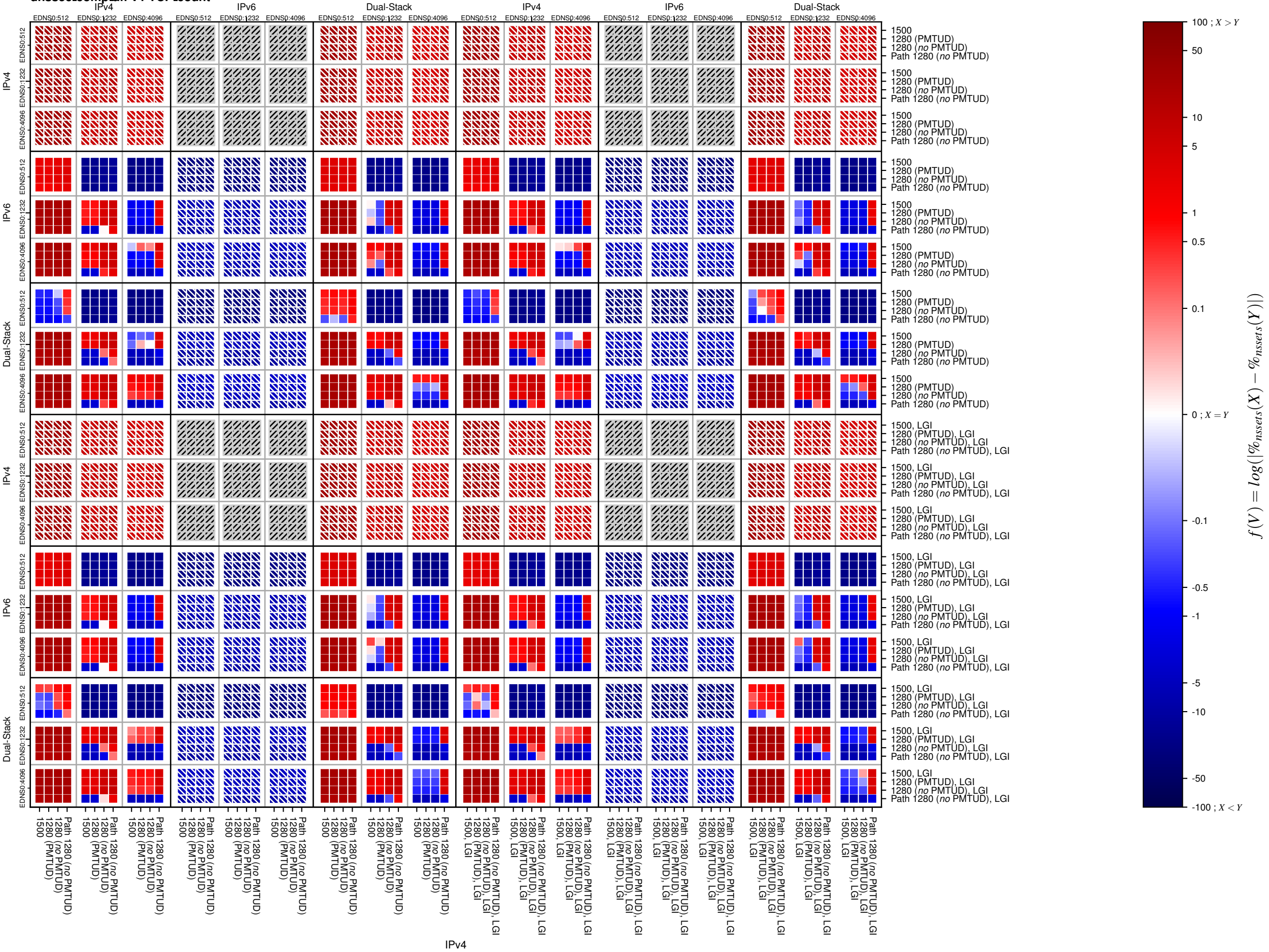
dnssec_comp_afv4-TCP_count
