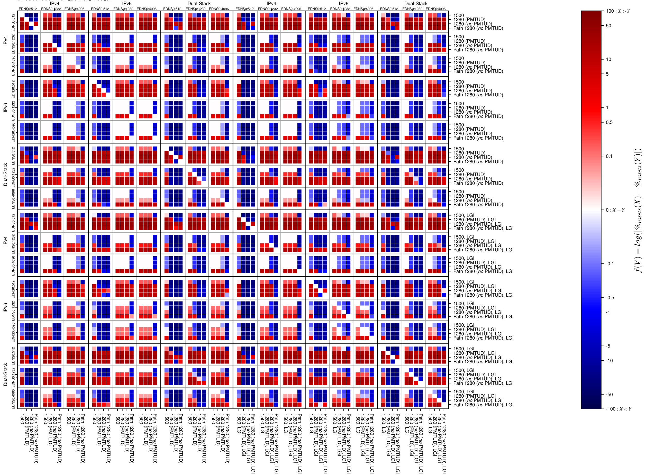
dnssec-both-TCP_server_mss_ok
