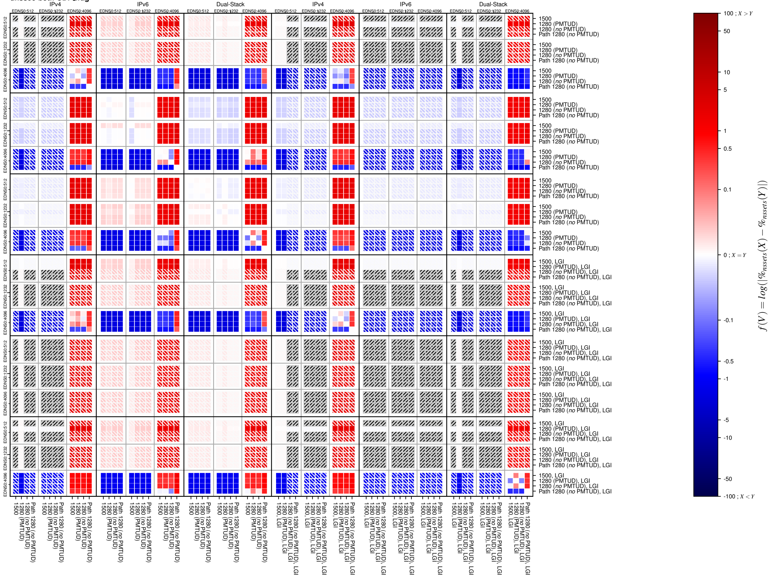
dnssec-both-UDP_frag
