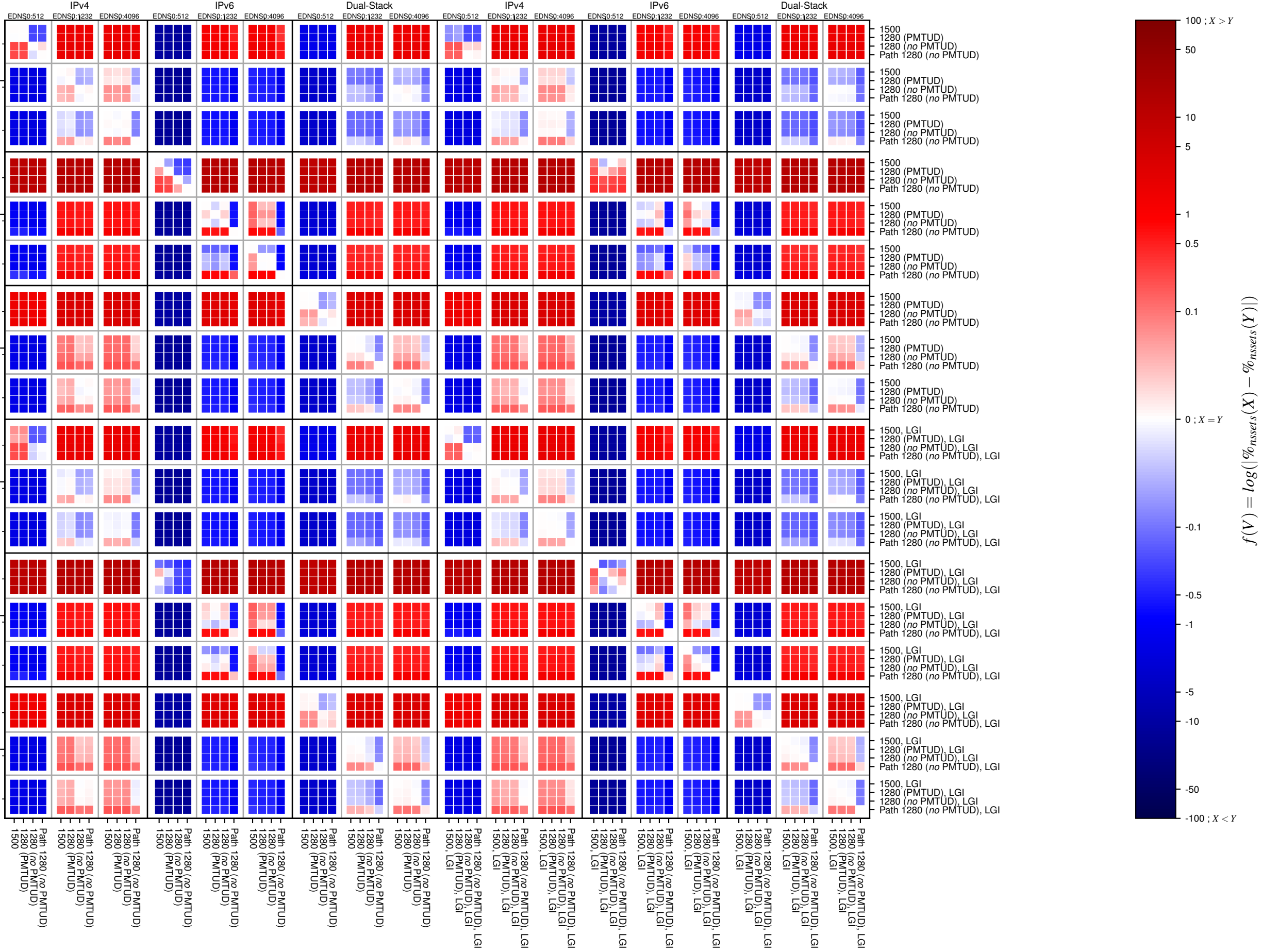
no_dnssec-both-UDP_count
