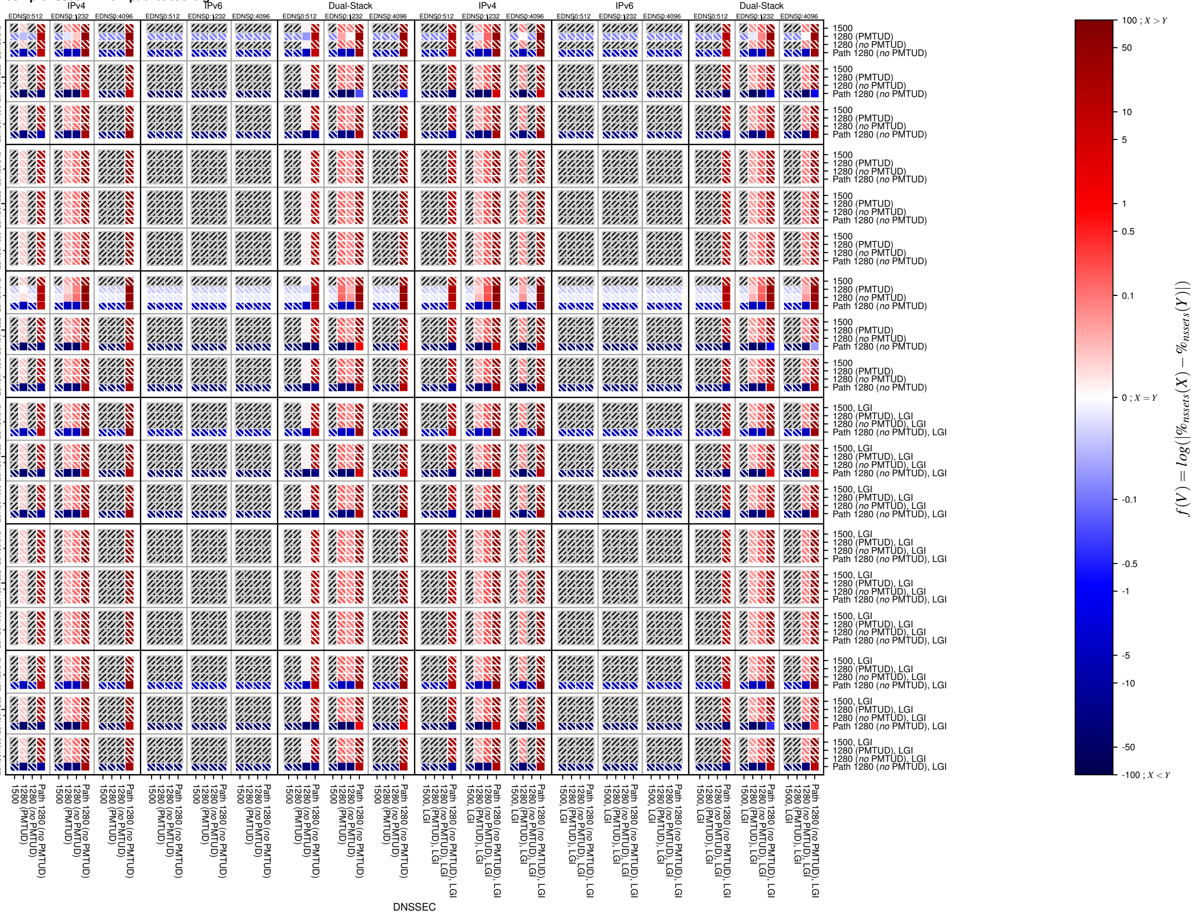
comp_dnsssec-v4-TCP_packet_too_big
