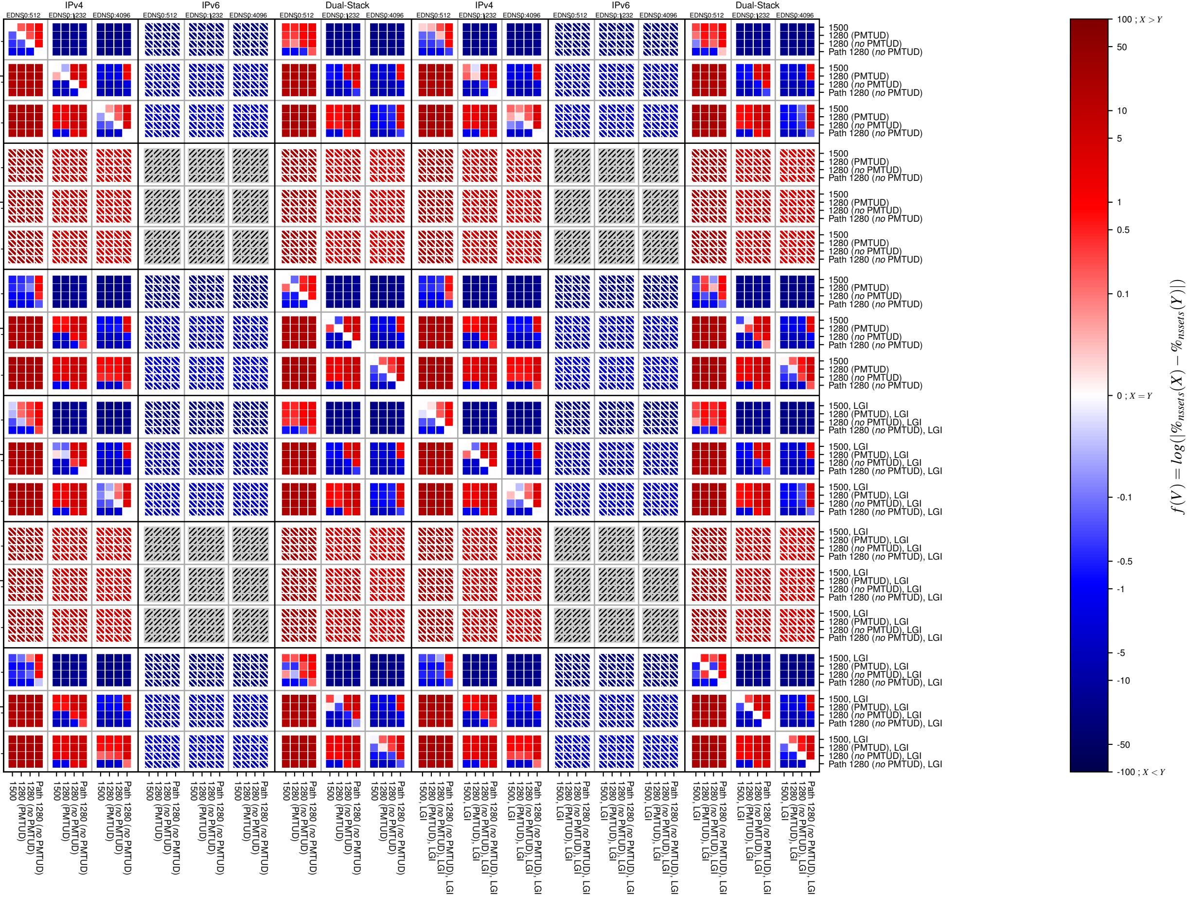
dnssec-v4-TCP_count
