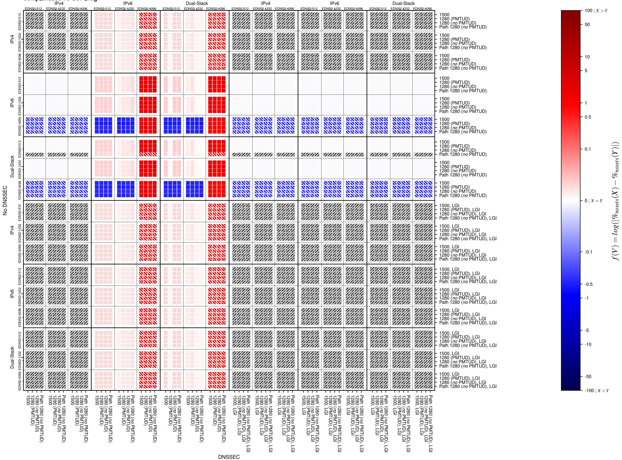
comp_dnsssec-v6-UDP_frag
