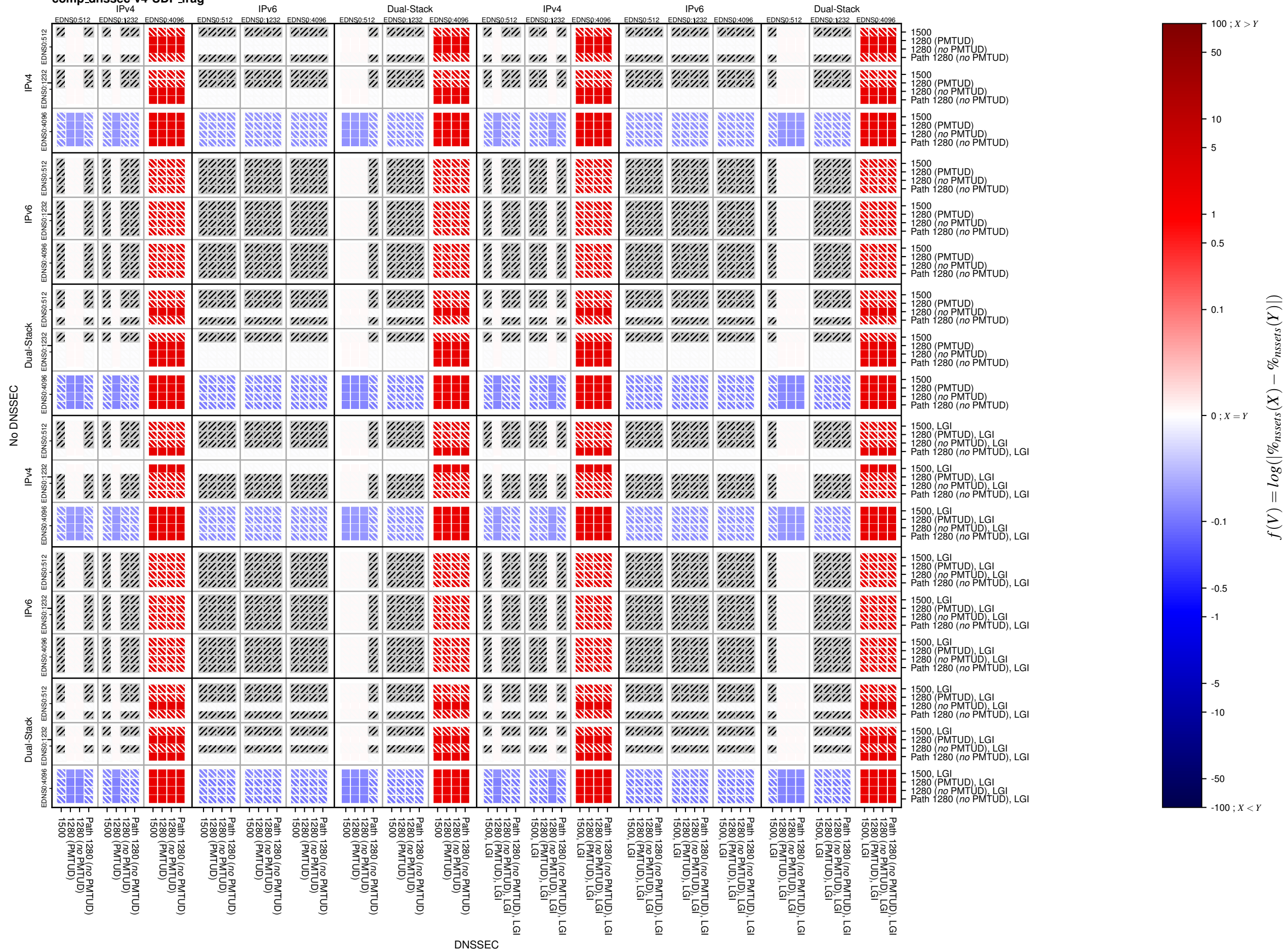
comp_dnsssec-v4-UDP_frag
